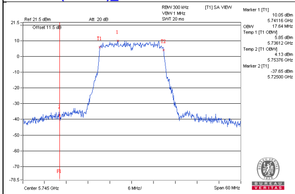
802.11ac(VHT20)_Chain2 / CH149
