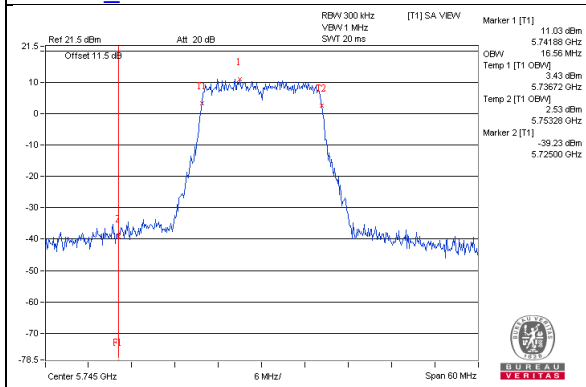
802.11ac(VHT20)_Chain0 / CH149
