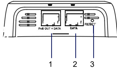
Figure 2: Bottom Connectors
