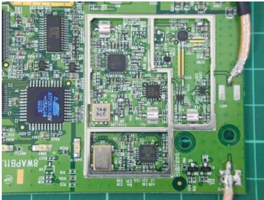
Photo 3: Internal photo of WAP-B11
