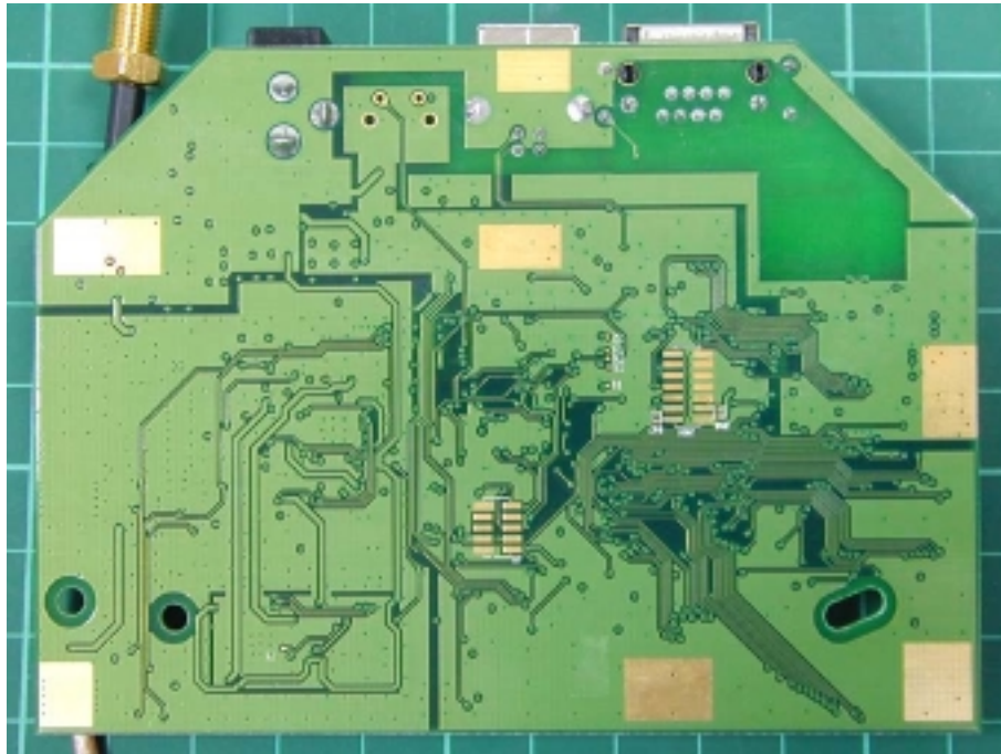
Photo 4: Internal photo of WAP-B11
