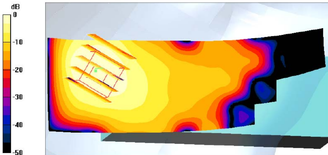
0 dB = 0.030\text{mW/g}
