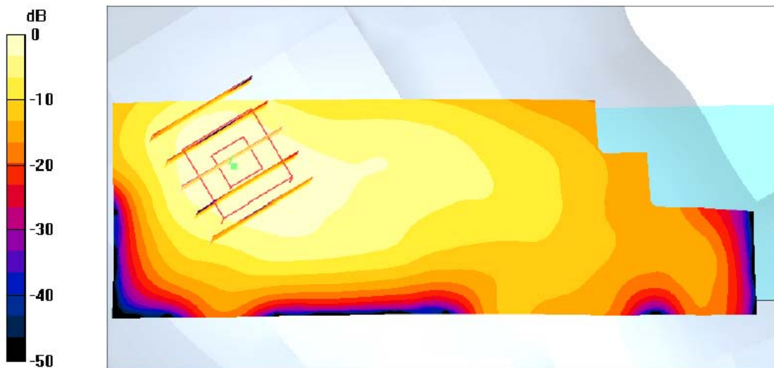
0 dB = 0.020mW/g
