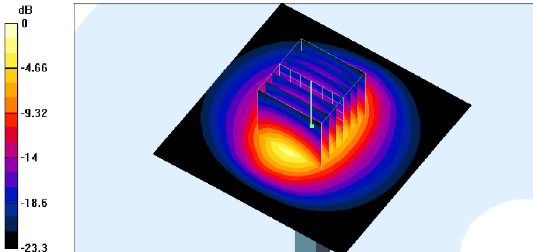
0 dB = 5.84mW/g
