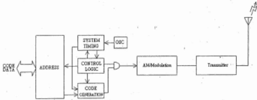
TX-1001-2T/4T BLOCK DIAGRAM
