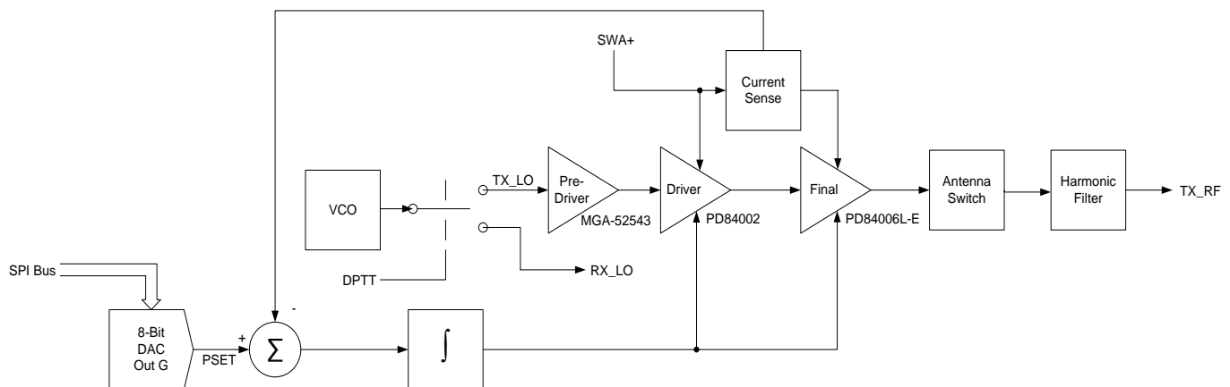
Figure 1 – Transmitter at Type Acceptance Grant
