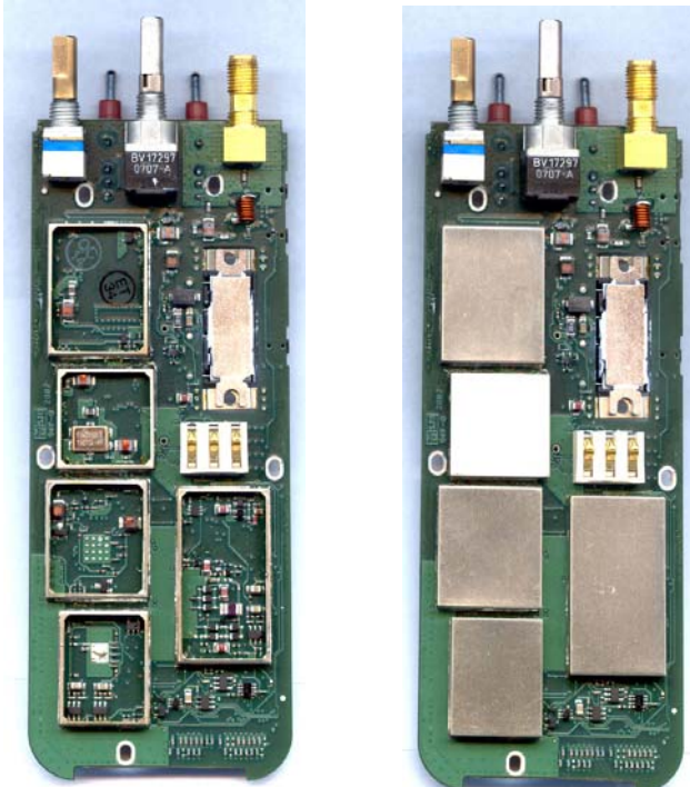
RF board bottom side.
