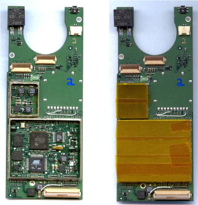
System board bottom side
