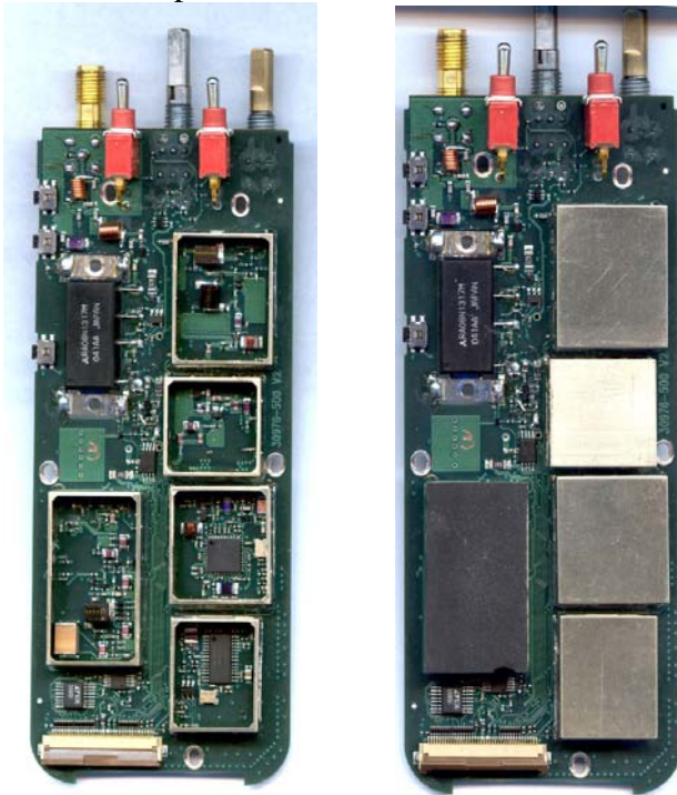
RF board top side
