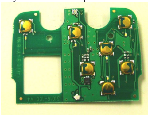
Keyboard board - Top side
