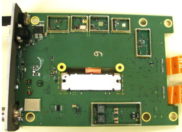
RF board - Bottom side.
