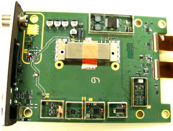
RF board - Top side
