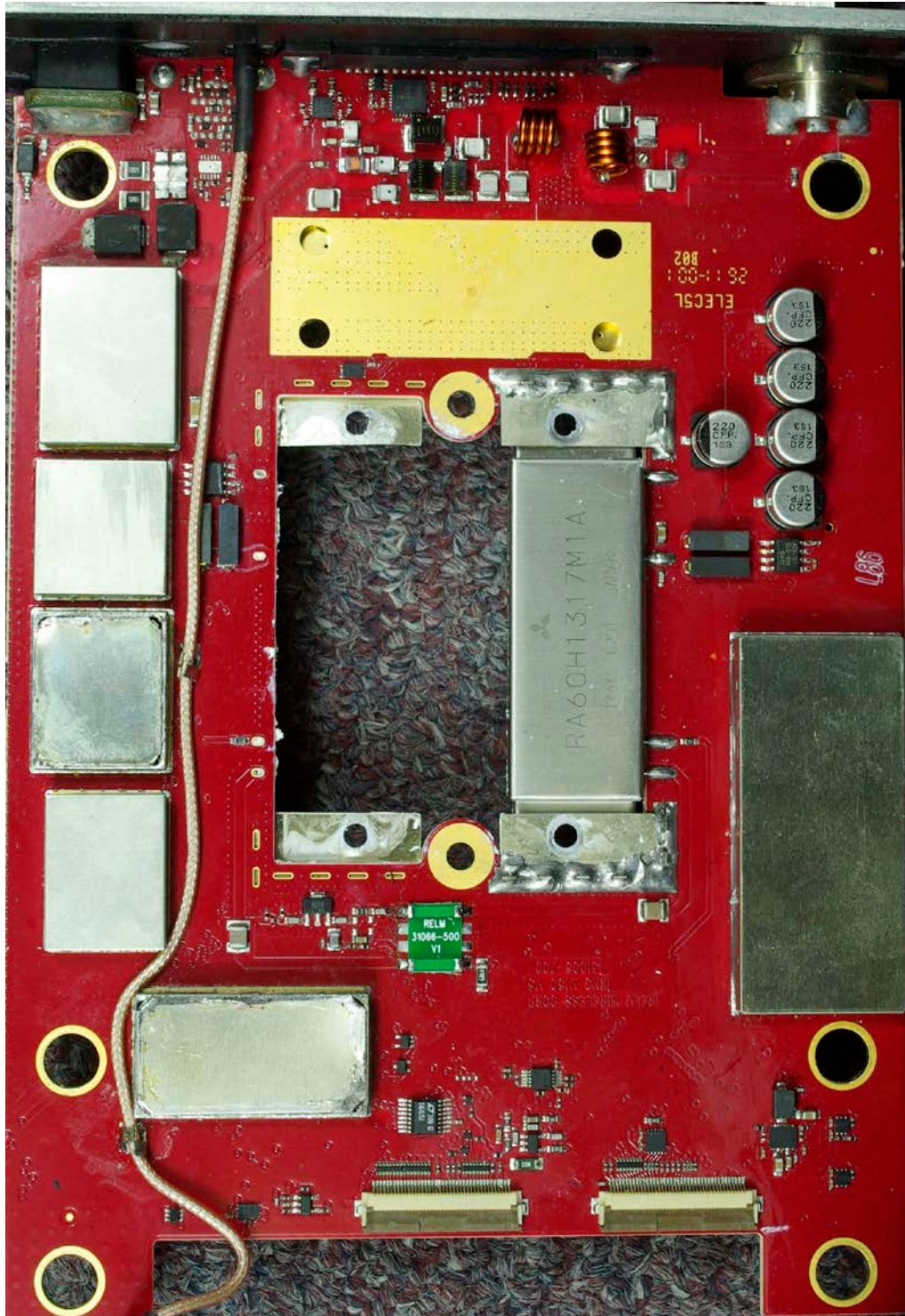
RT TOP WITH SHIELDS
