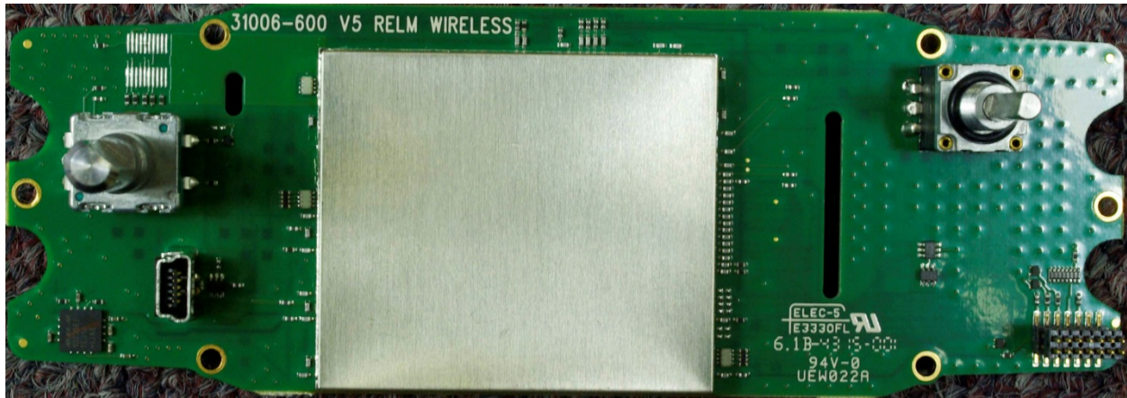
SYSTEMS BOARD – TOP WITH SHIELDS
