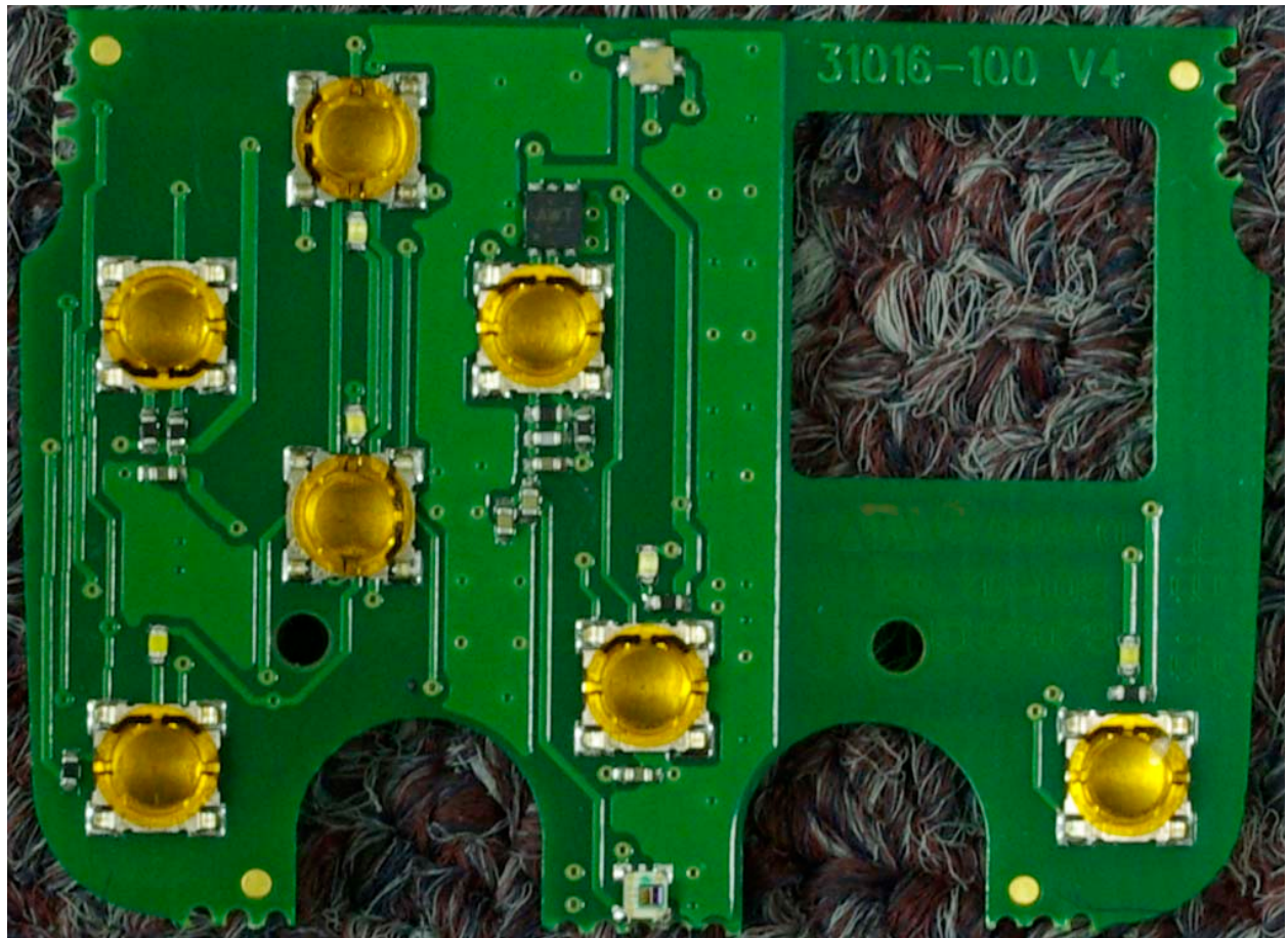
KEYBOARD – TOP
