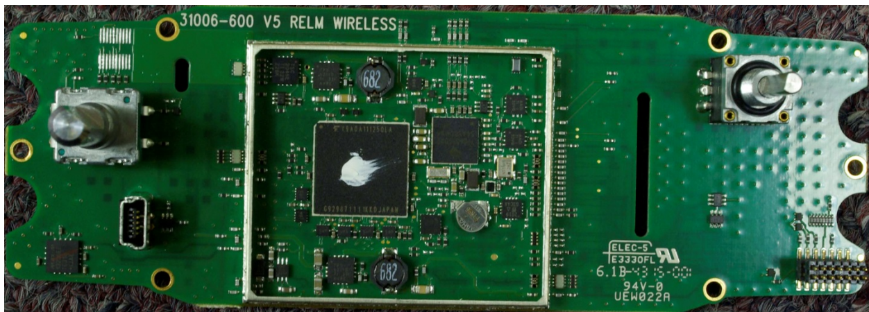
SYSTEMS BOARD –TOP WITH NO SHIELDS
