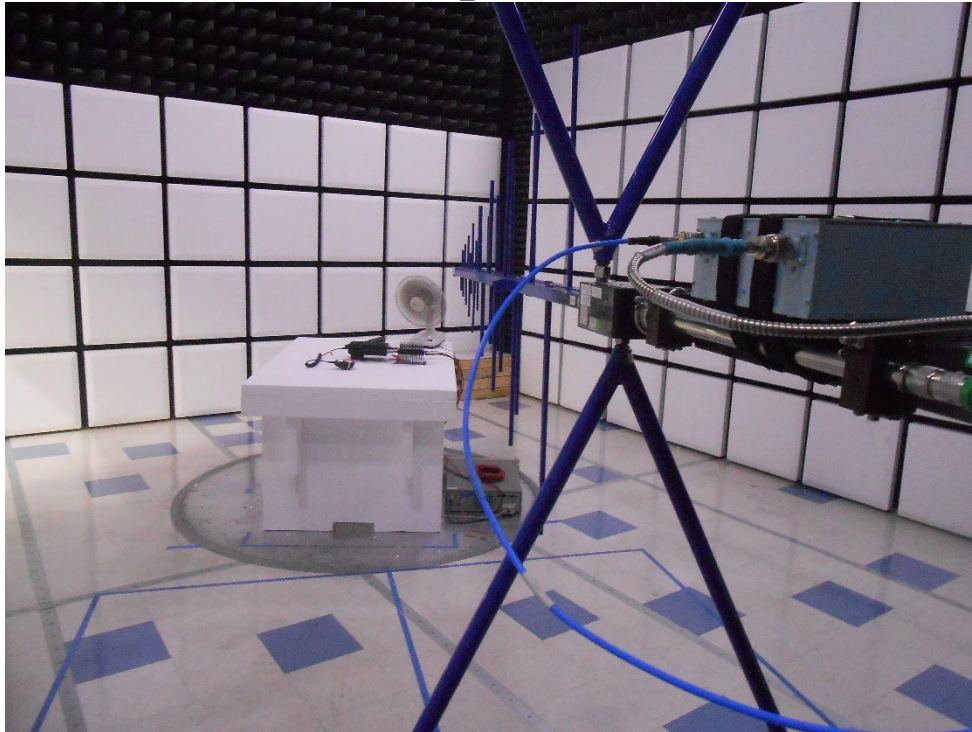
RF Radiated_ below 1 GHz #1
