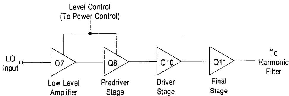
Power Amplifier Block Diagram
