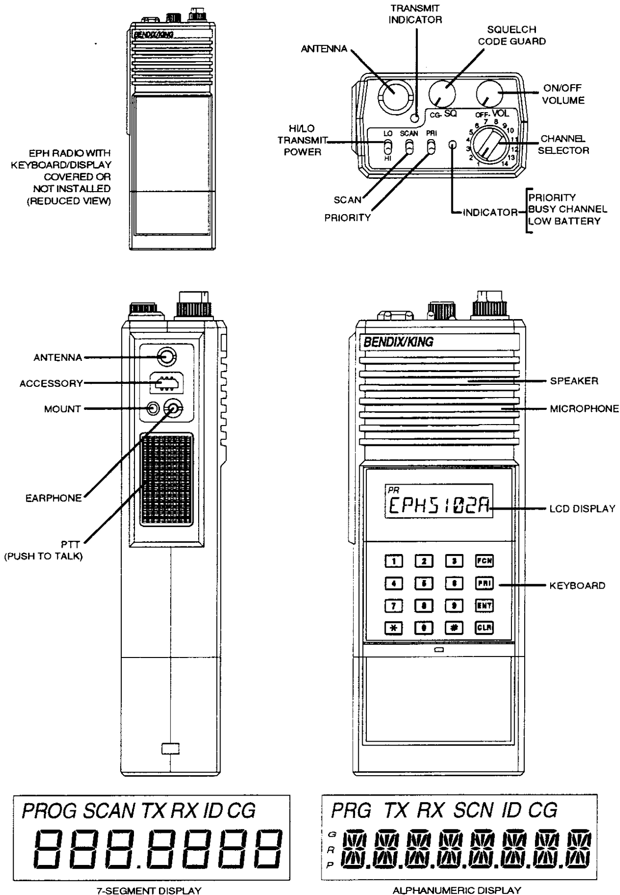
FIGURE 1-1 CONTROLS
