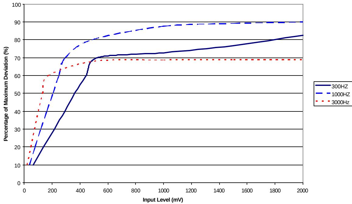
Percent Modulation vs. Input level 25KHz Channel 161.5MHz
