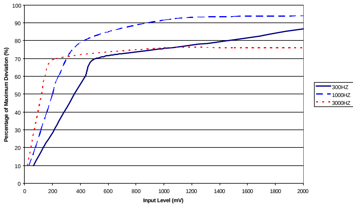
Percent Modulation vs. Input Level 12.5KHz Channel 161.5MHz
