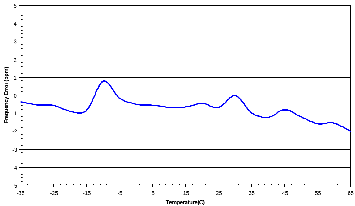
Frequency Error vs. Temperature FCC Limit +/-5ppm
