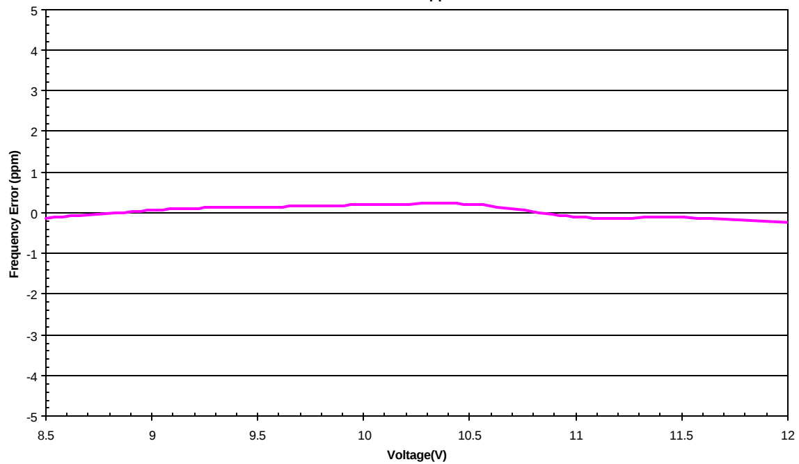
Frequency Error vs. Voltage @25C FCC Limit +/-5ppm
