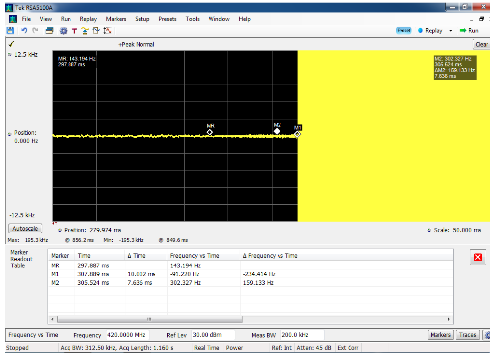
Transient Freq Behavior_420 MHz_T on
