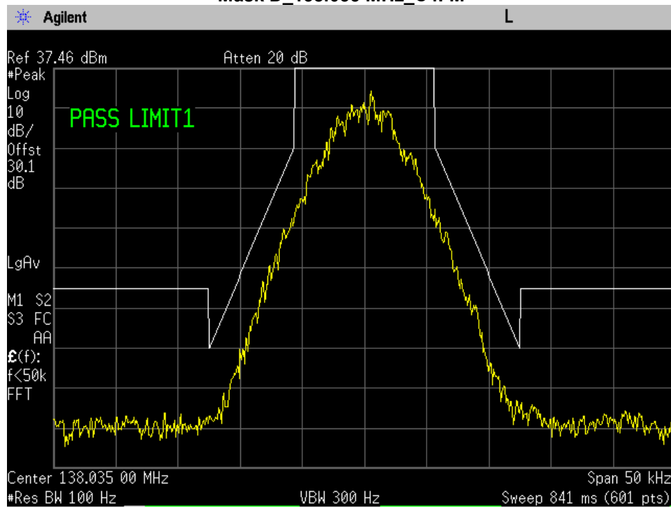
Mask D_138.035 MHz_C4FM
