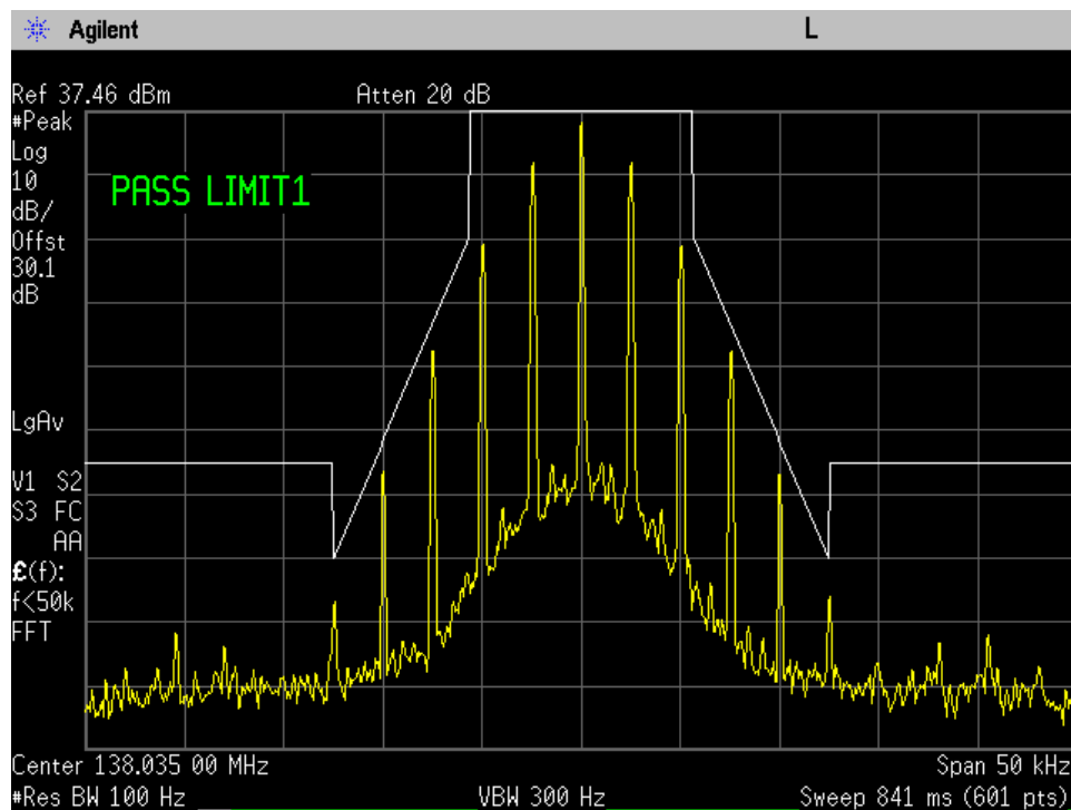
Mask D_138.035 MHz_NB
