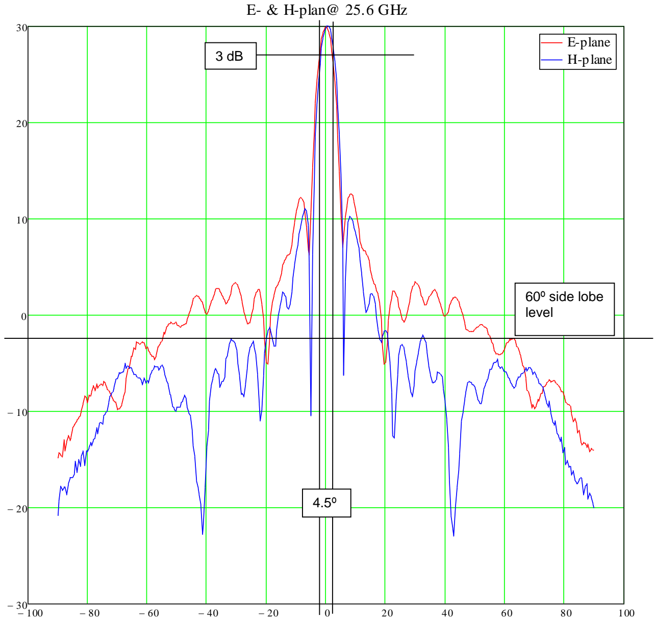
Antenna diagram (Gain in dBi).
