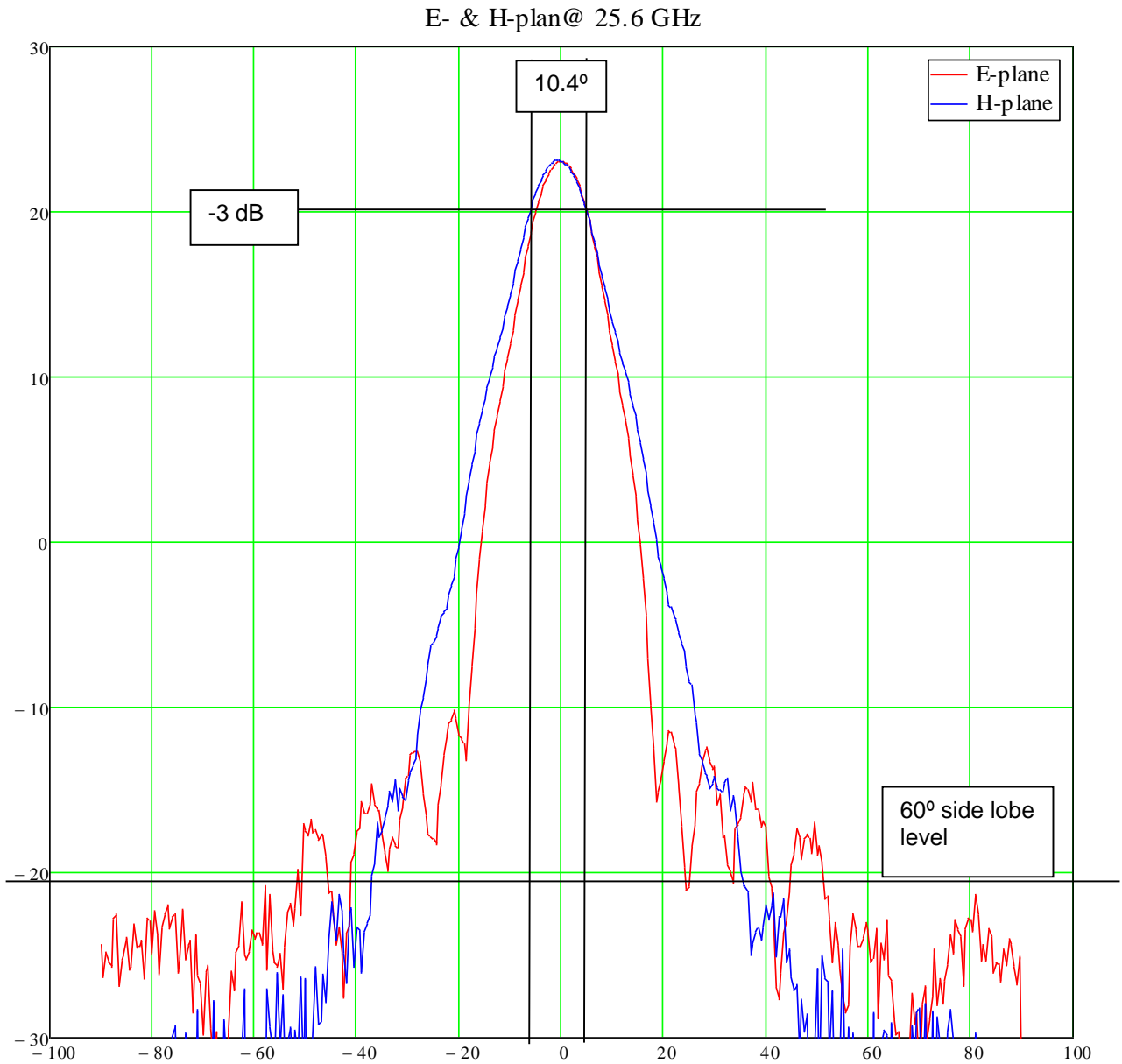
Antenna diagram (gain in dBi): 4 inch horn antenna.
