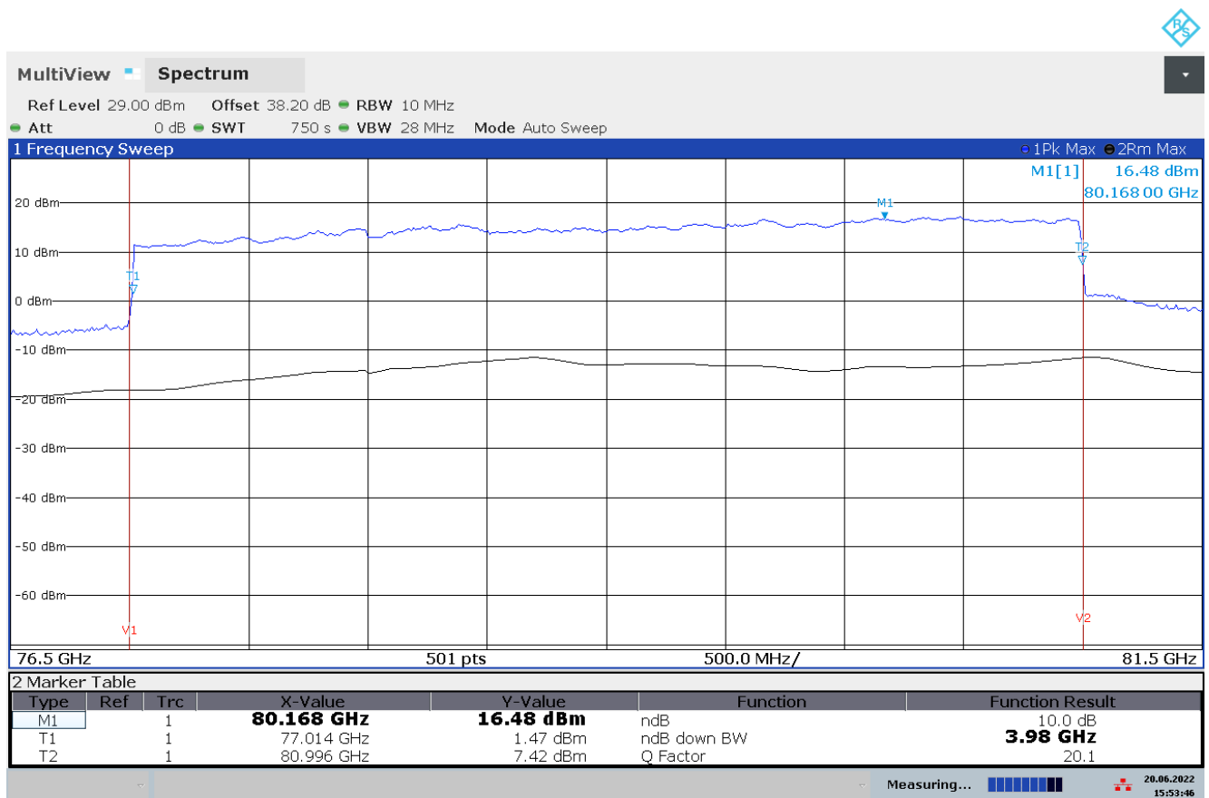
Plot 1: 10 dB bandwidth, Pos-Peak measurement, reference at 20°
