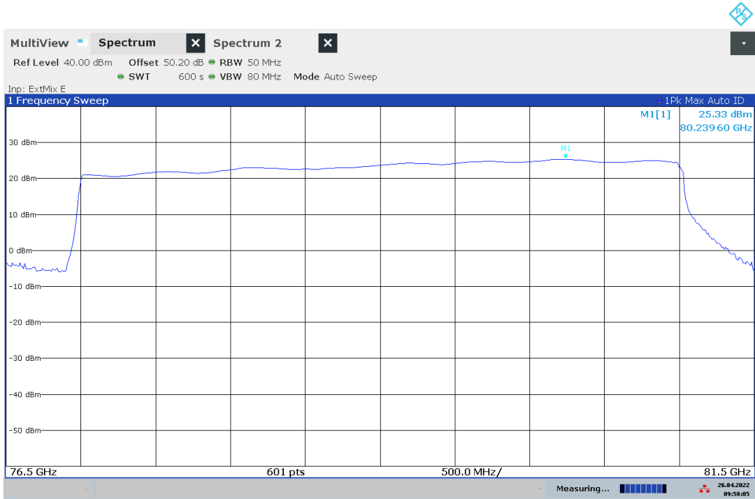
Plot 2: Peak EIRP
