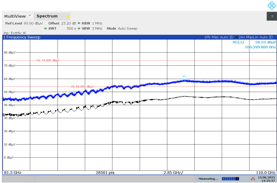
Plot 11: 81 GHz – 110 GHz, PEAK/RMS-measurement
