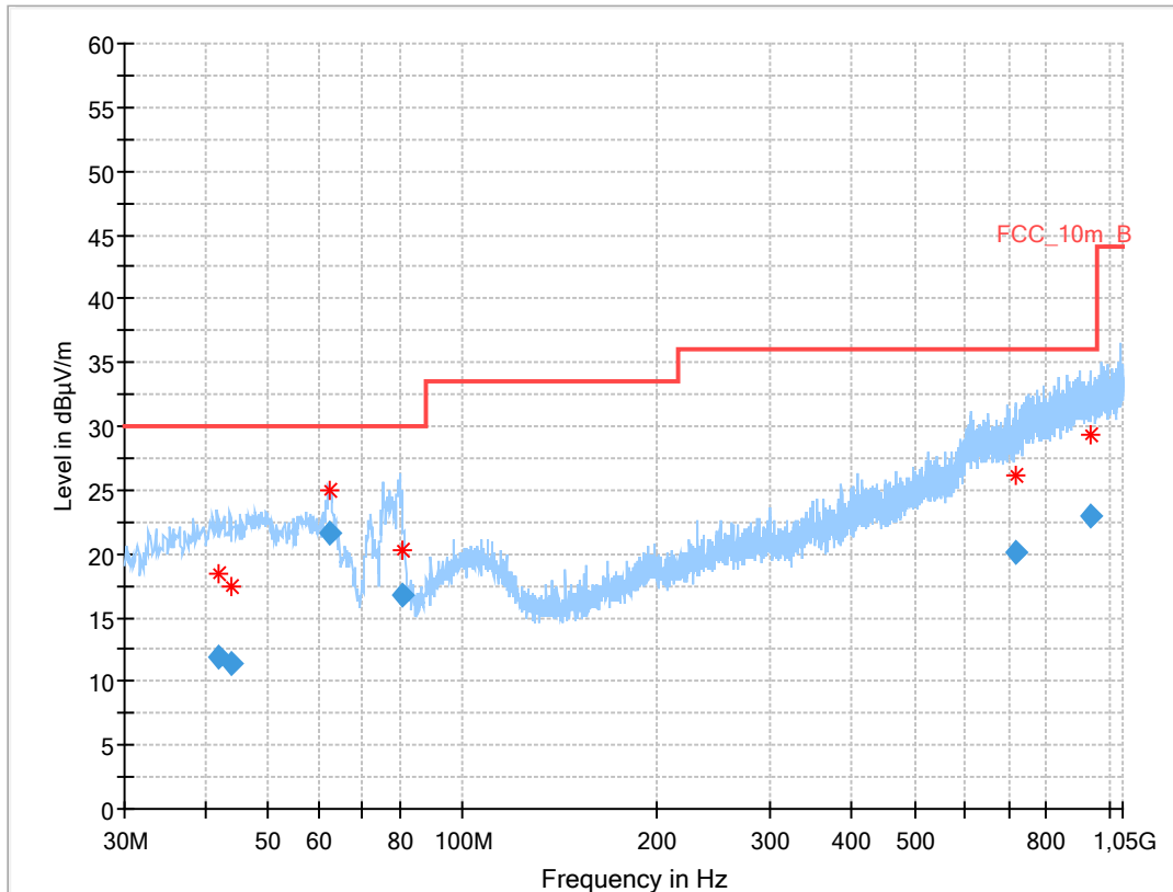
Plot 2: 30 MHz to 1 GHz, TX mode, 2440 MHz, vertical & horizontal polarization, valid for all channels of 2 Msps
