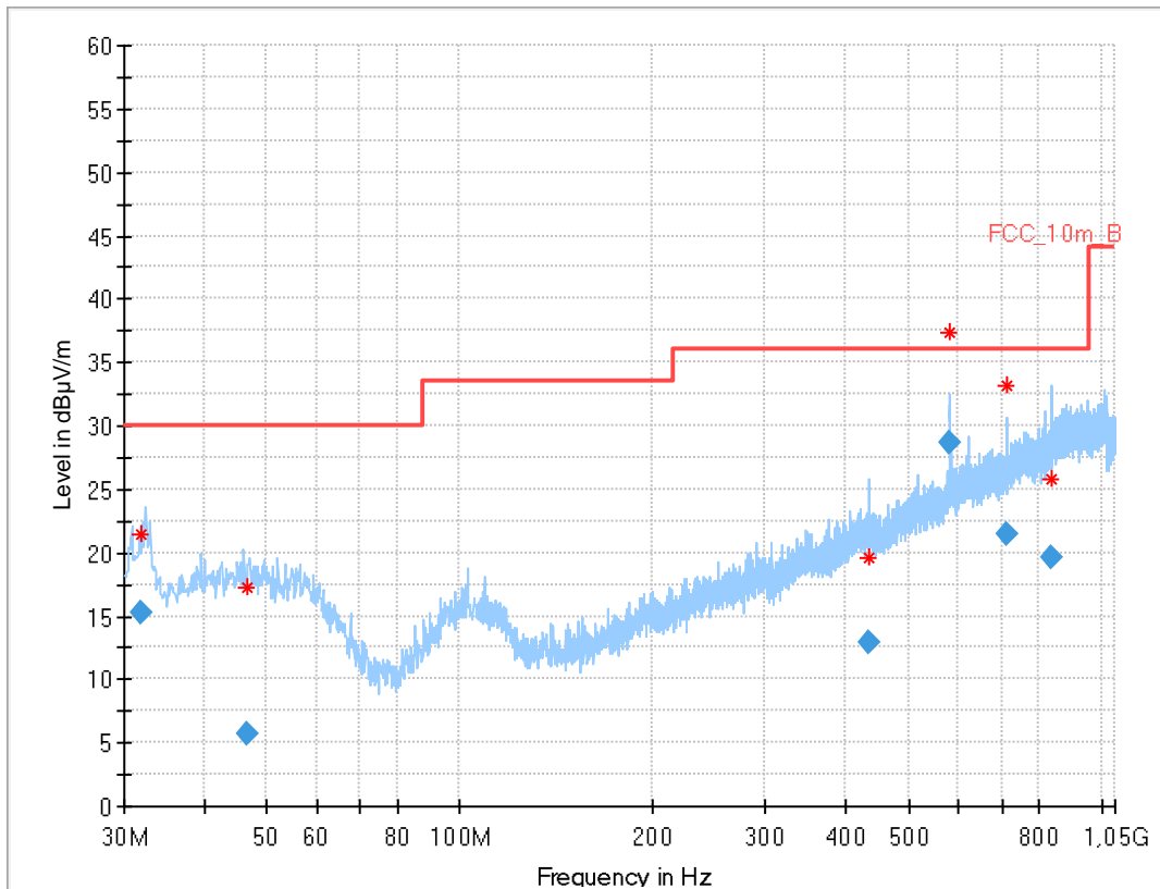
Plot 4: 30 MHz – 1000 MHz, special test mode, f high
