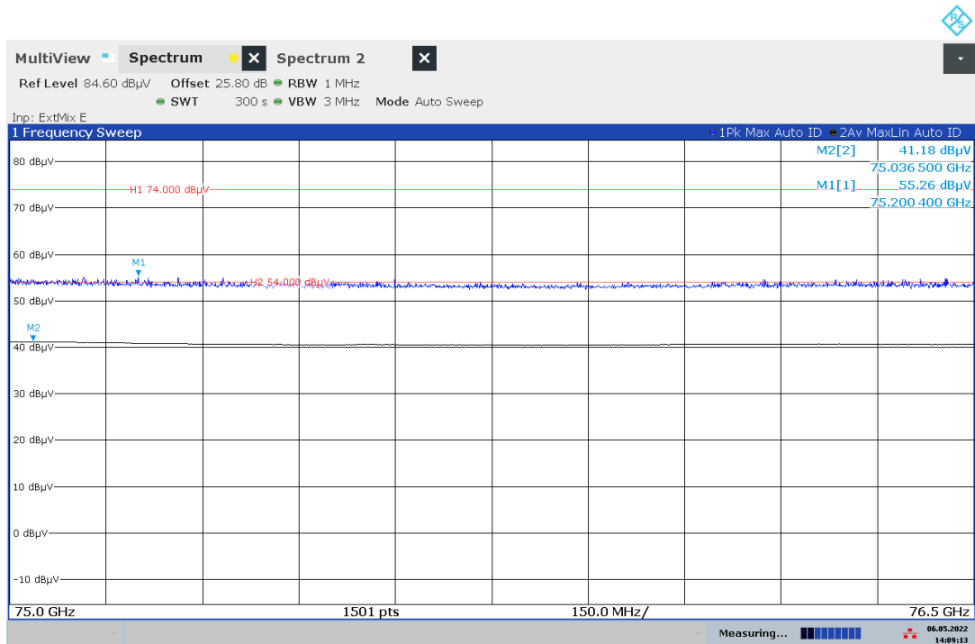
Plot 11: 75 GHz – 76.5 GHz, PEAK/RMS-measurement, f_{low}/f_{mid}/f_{high}
