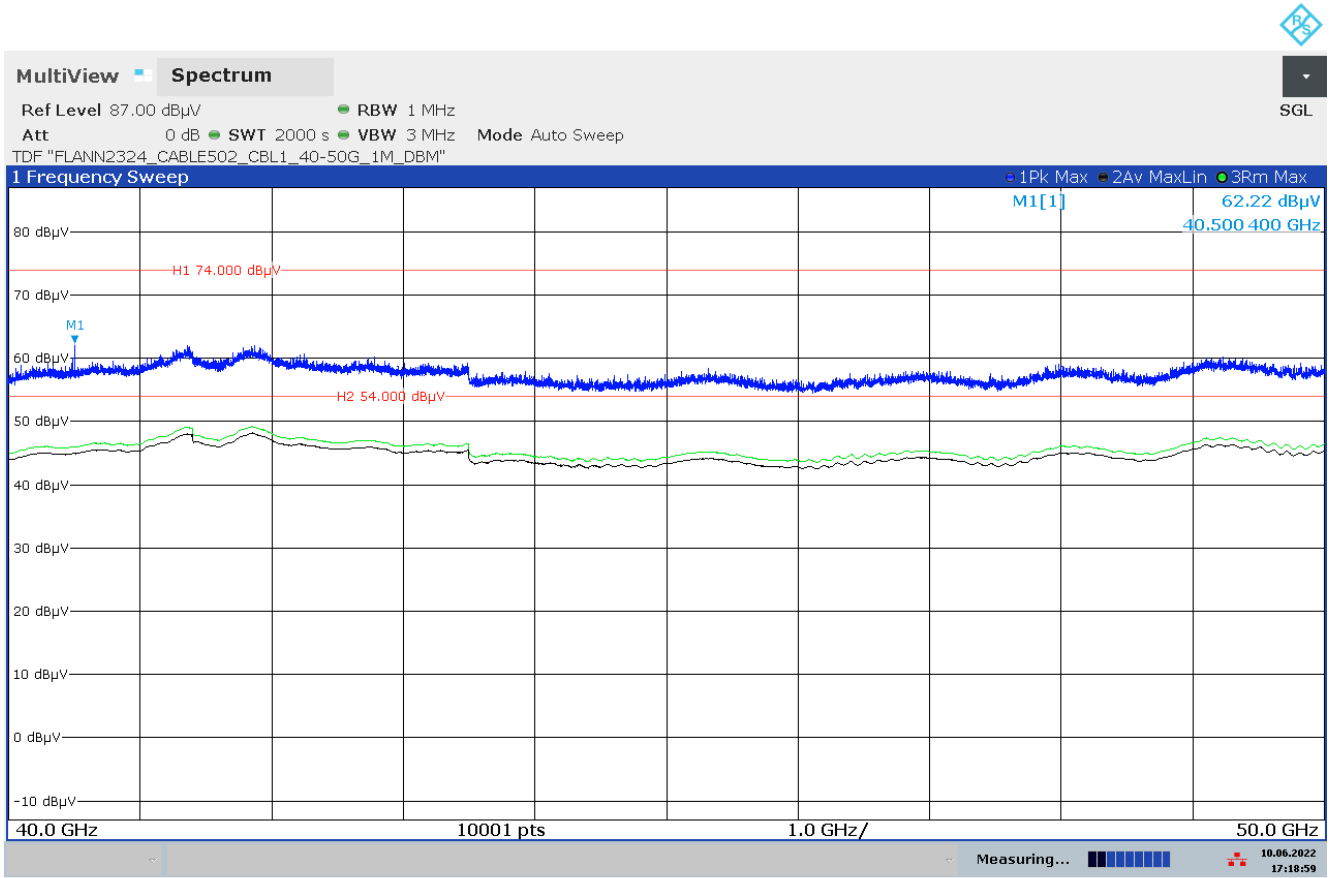
Plot 9: 40 GHz – 50 GHz, PEAK/RMS-measurement, f_{low}/f_{mid}/f_{high}
