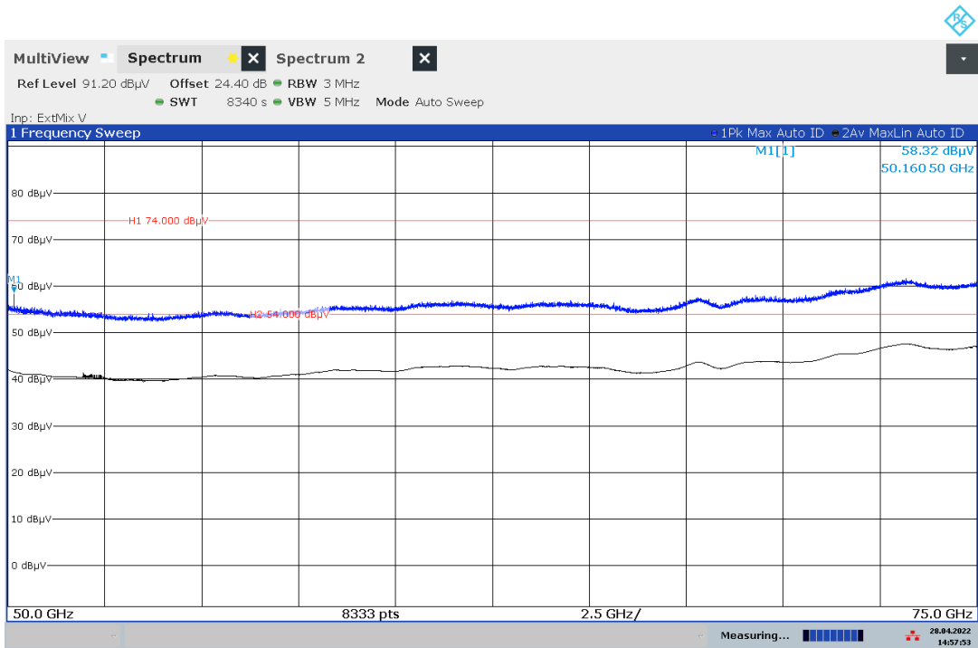
Plot 10: 50 GHz – 75 GHz, PEAK/RMS-measurement, f_{low}/f_{mid}/f_{high}
