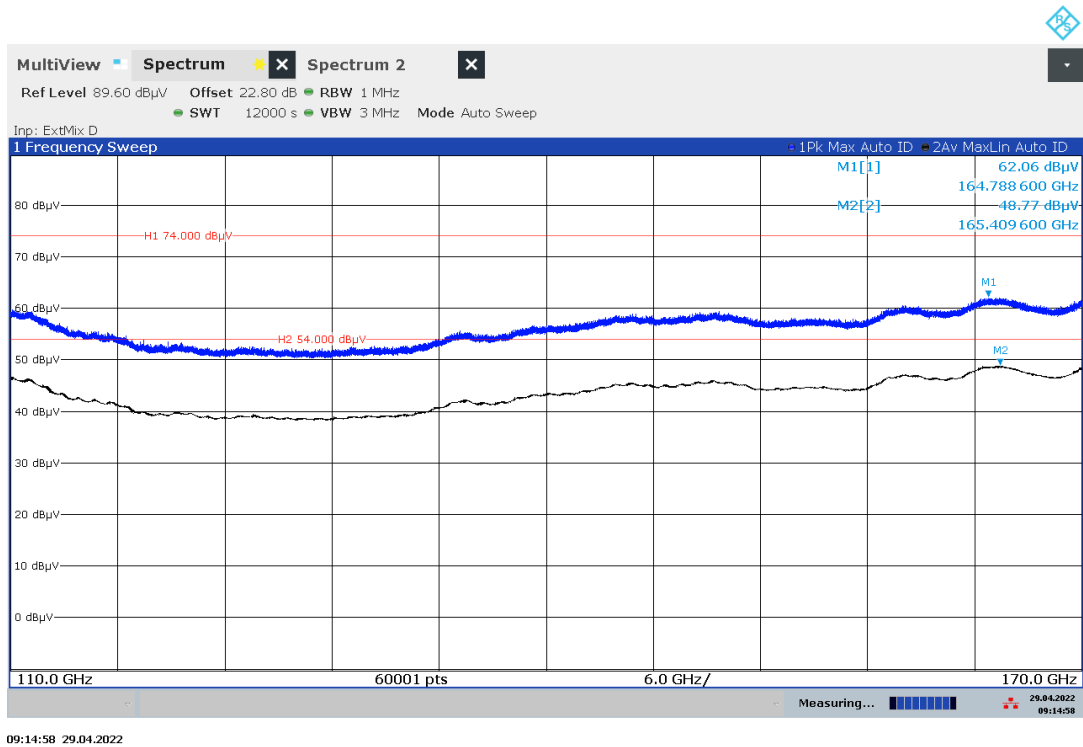
Plot 15: 110 GHz – 170 GHz, PEAK/RMS-measurement, f_{low}/f_{mid}/f_{high}
