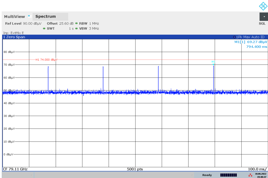
Plot 13: 79.1 GHz, PEAK/RMS-measurement, f_{mid} , Zero Span
