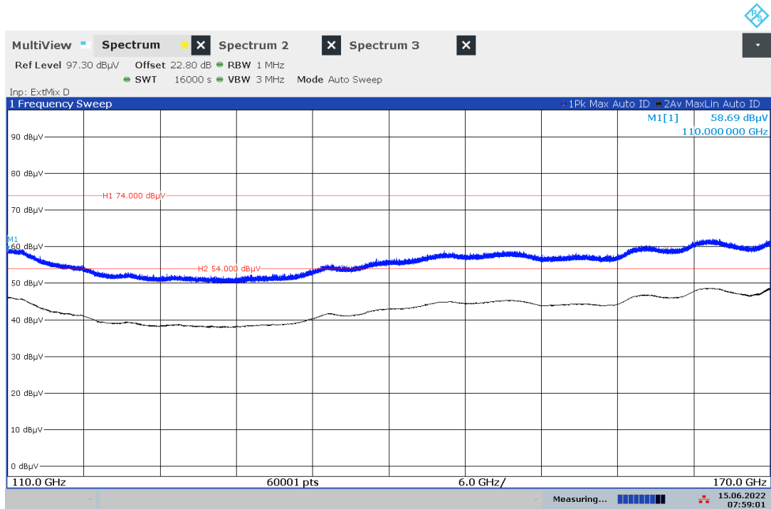
Plot 14: 110 GHz – 170 GHz, PEAK/RMS-measurement
