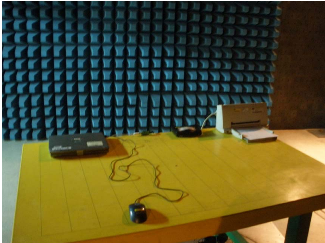
Photo 2: Radiated Emission Test set-up photo (WiFiHU-c-2-NE)
