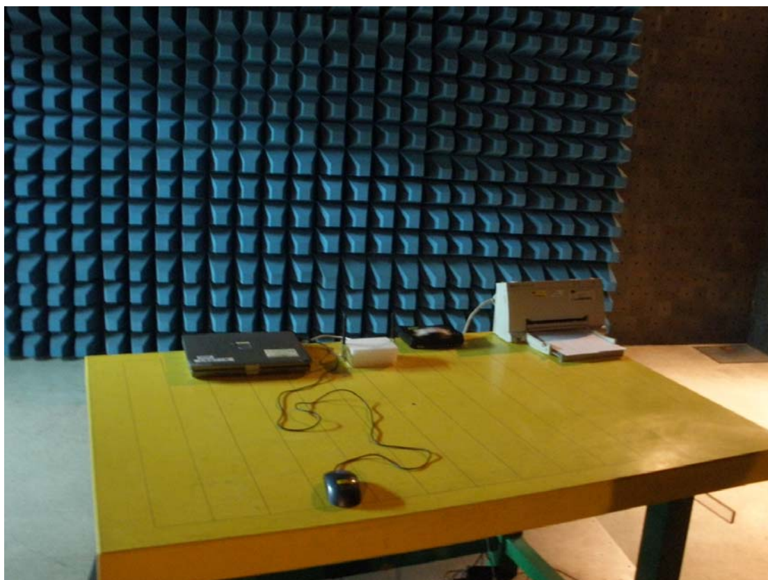
Photo 4: Radiated Emission Test set-up photo (WiFiHU-c-1-NE)
