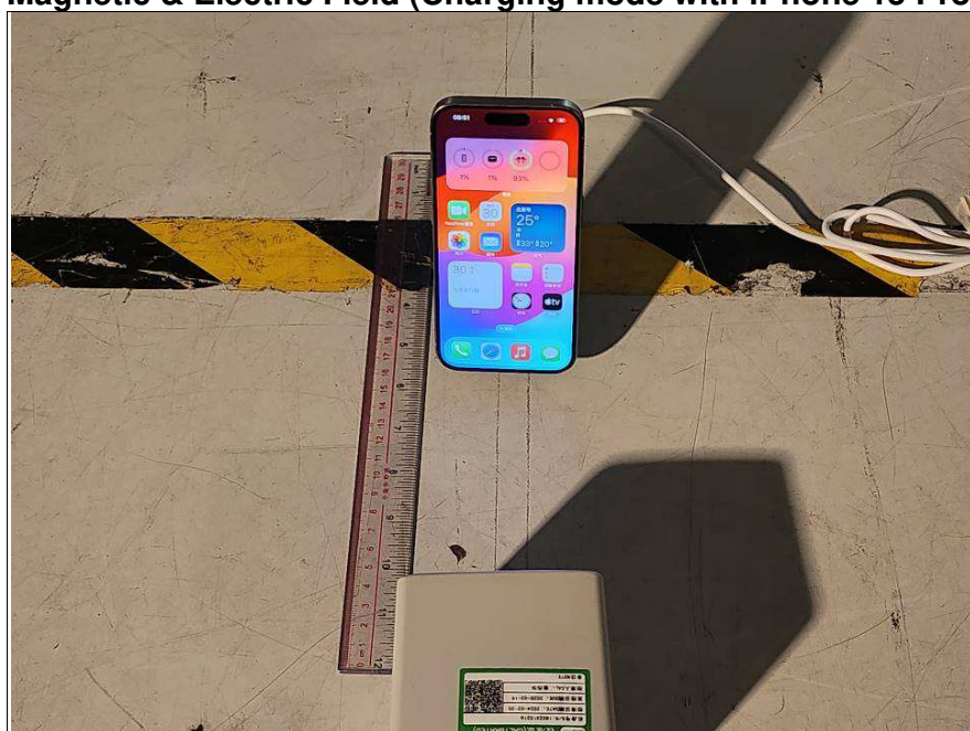
Magnetic & Electric Field (Charging mode with iPhone 15 Pro)
