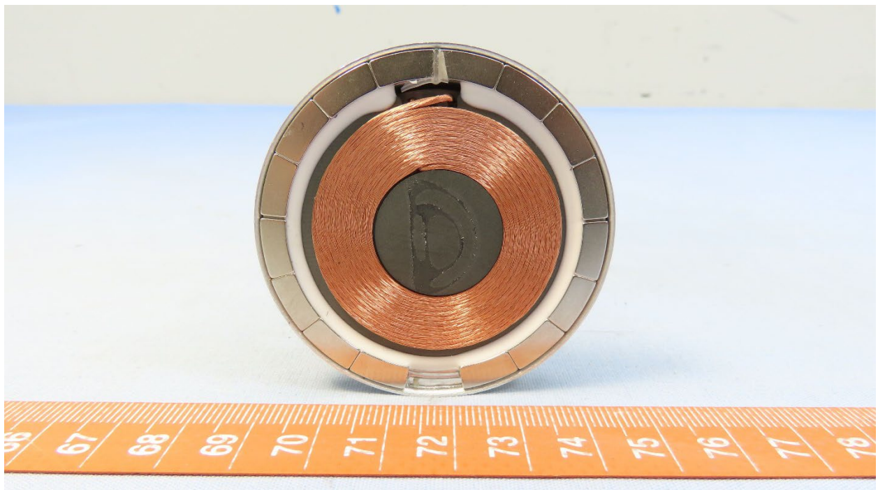
Qi2 Coil (Top Side)
