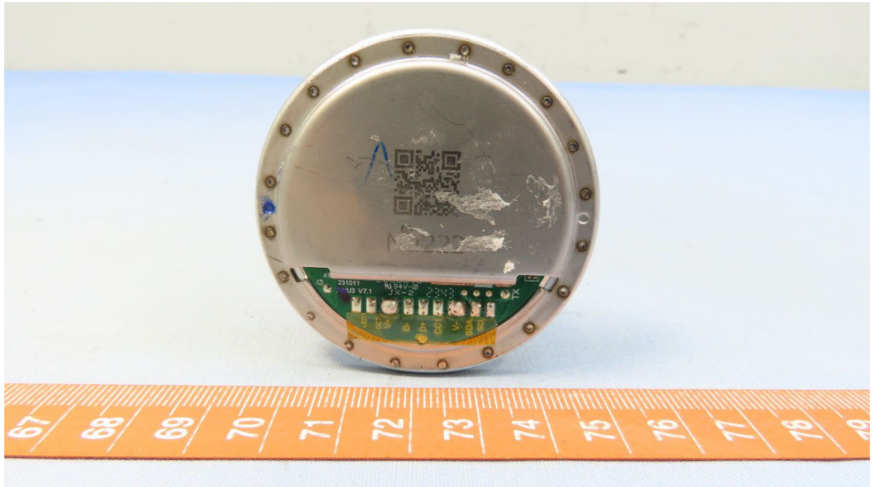
Qi2 Coil (Bottom Side)
