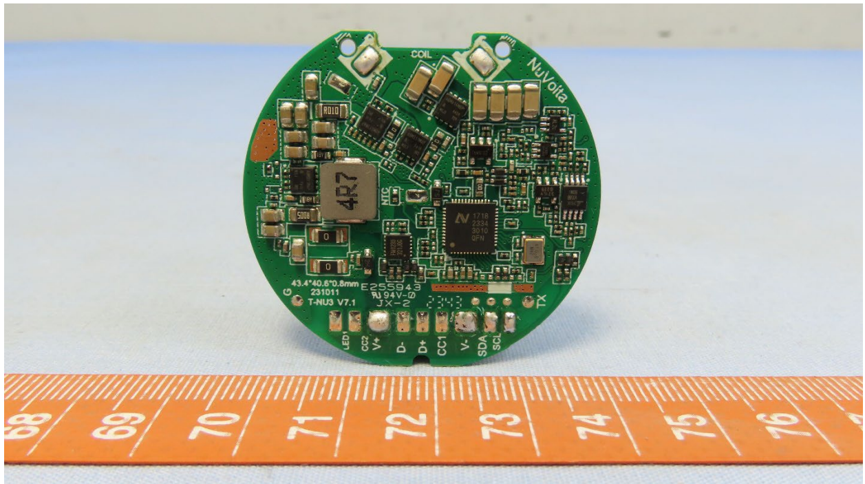
Qi2 PCBA (Bottom Side)
