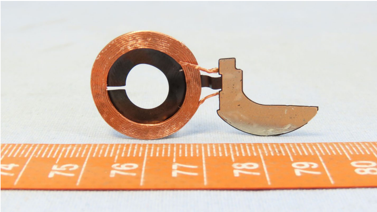
Apple Watch Coil (top side)
