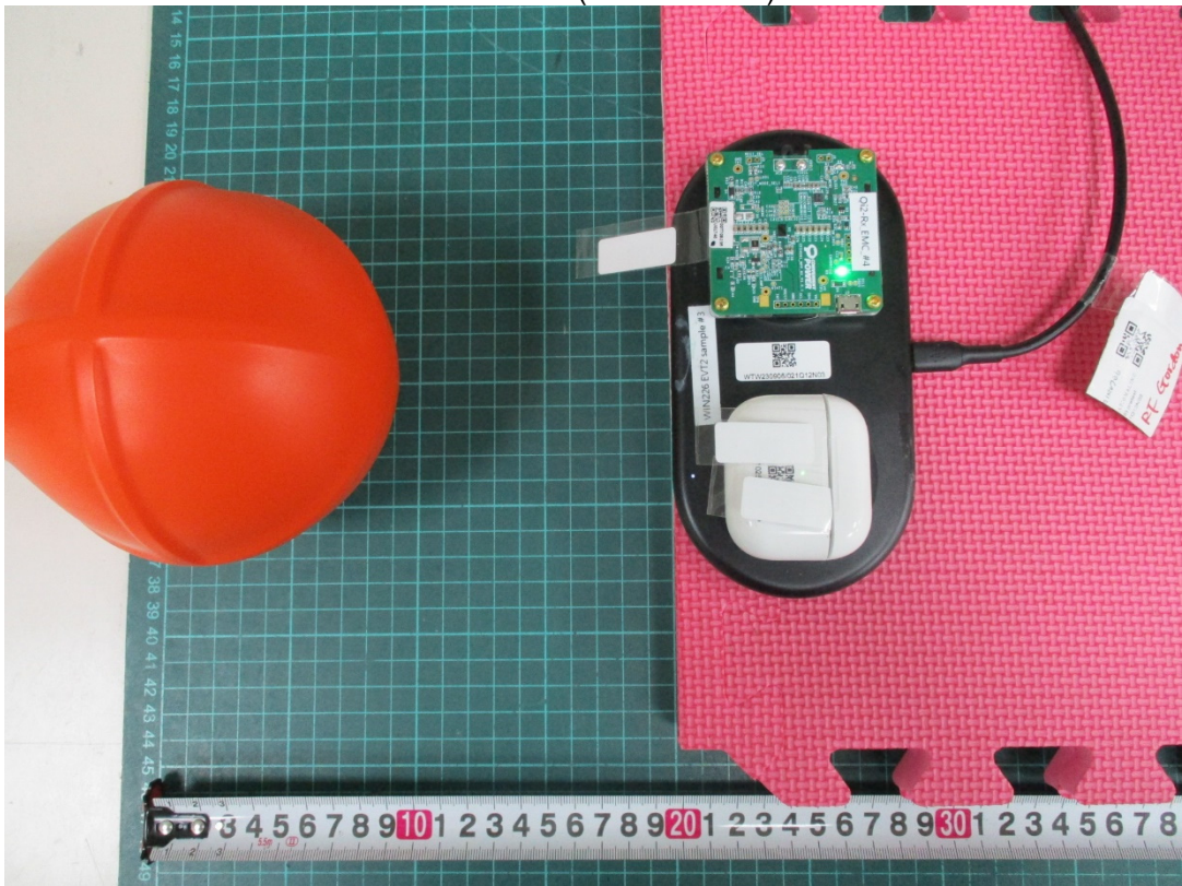
Test Mode F (Bottom: 20cm)
