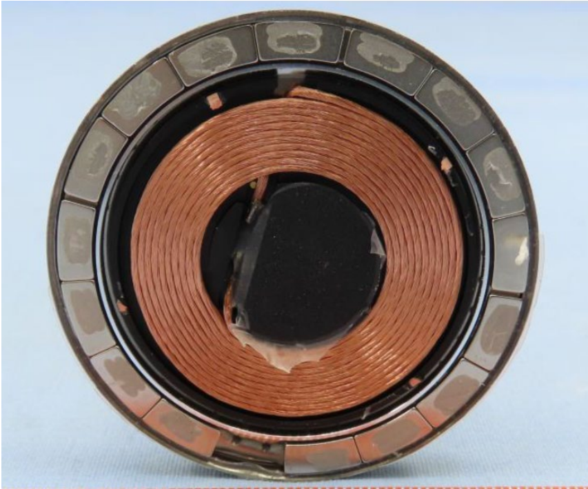
C222x Coil Antenna (MagSafe iPhones – 360 kHz) – Top View
