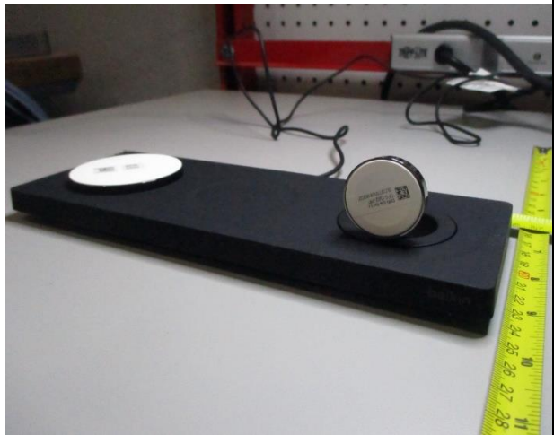
Angle view without inner base elevated, charging pad tilted upright
