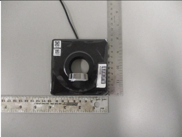
Top view with inner base elevated, charging pad tilted upright
