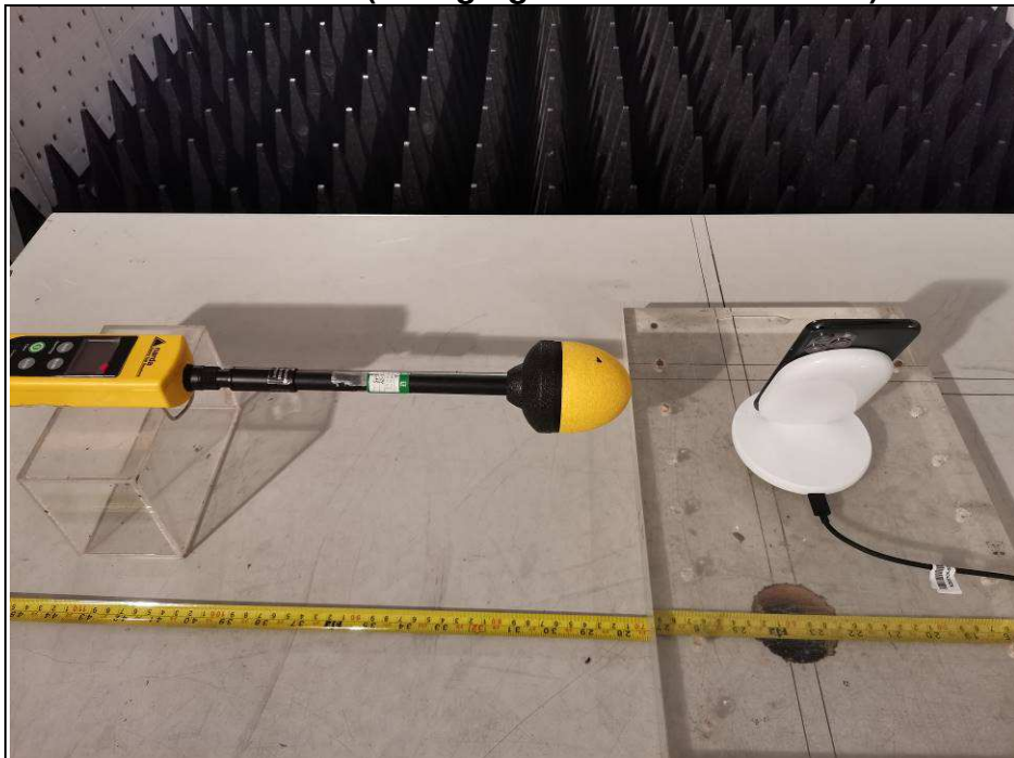
Electric Field(Charging mode with iPhone X)
