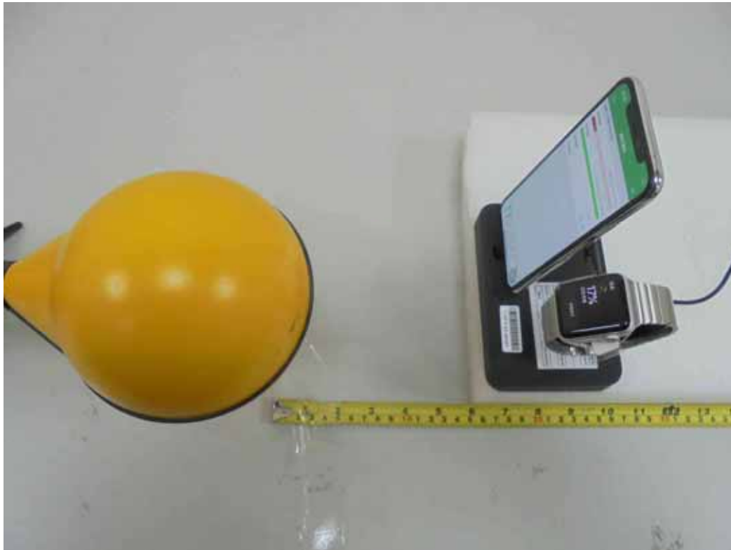
H-Field (Charging Mode with Apple Watch - Bottom)
