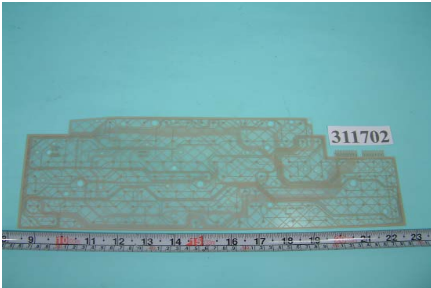
Front side of menbrane
