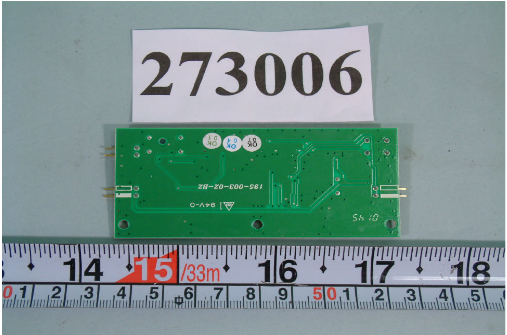
REAR side of Main Board Of Keyboard
