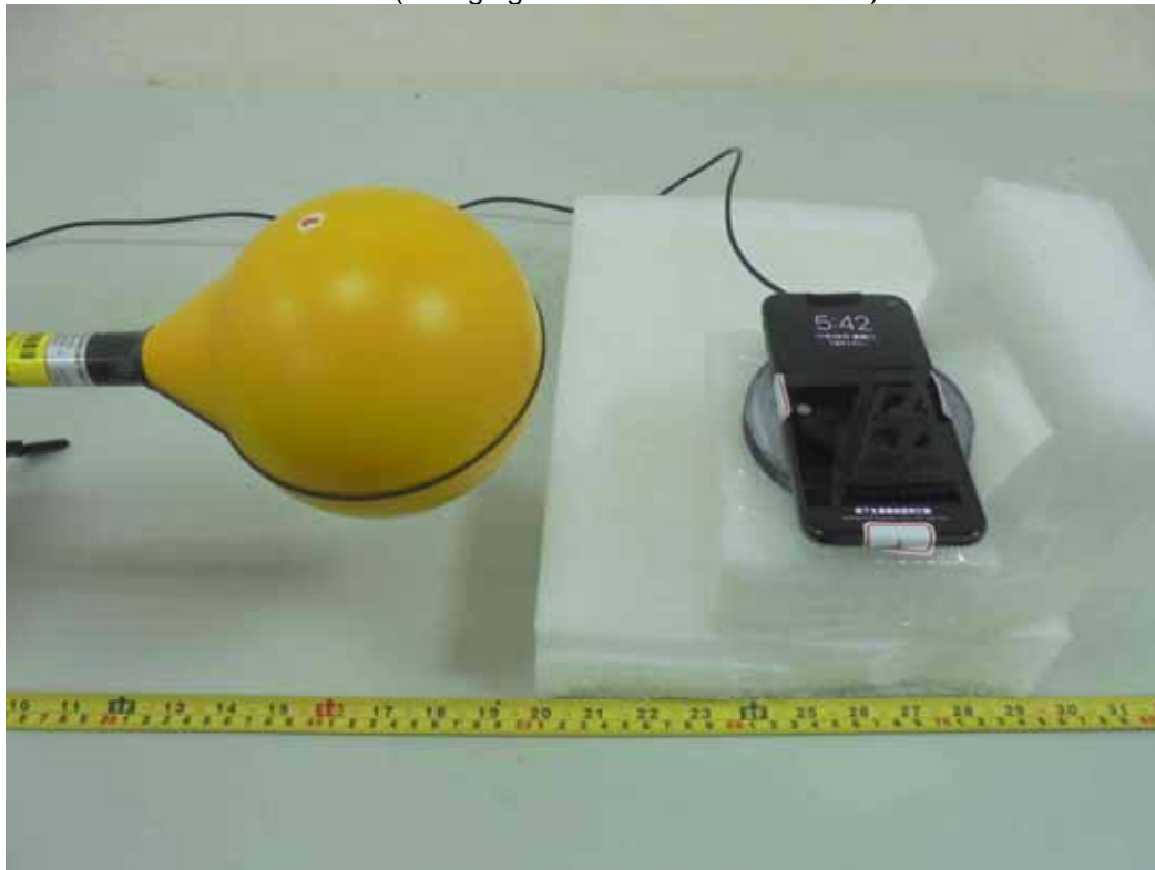
H-Field (Charging Mode with iPhone X - Right)
