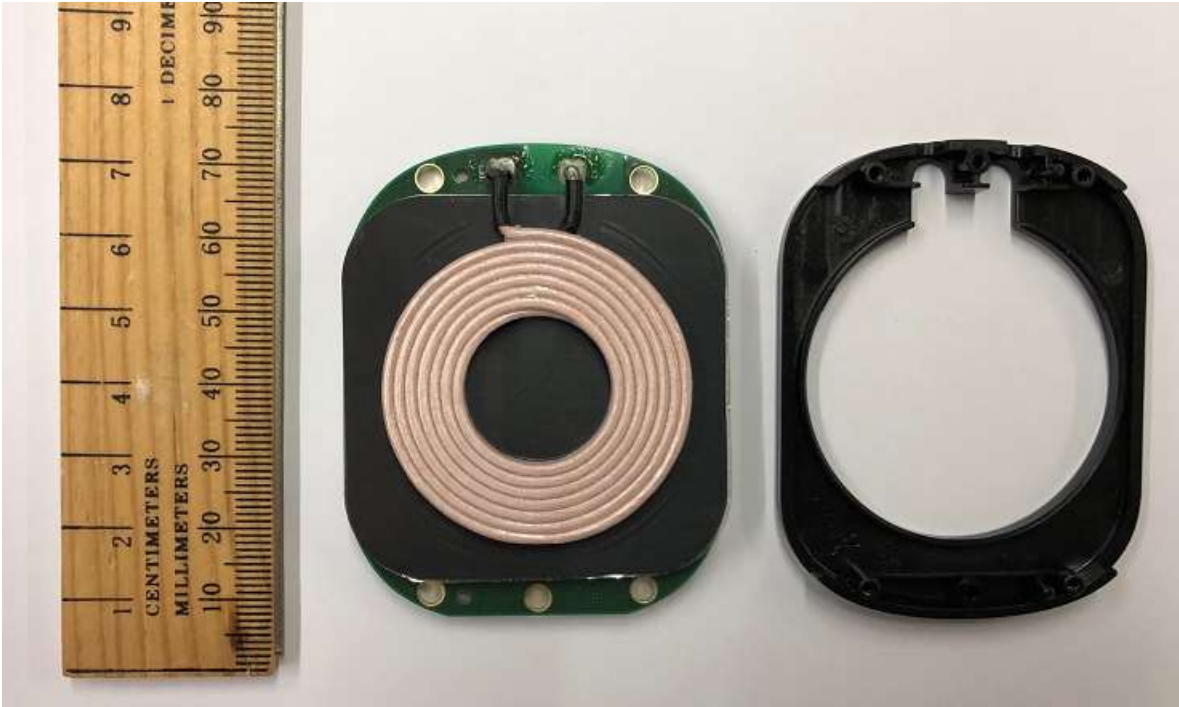
PCB Front side with coil
