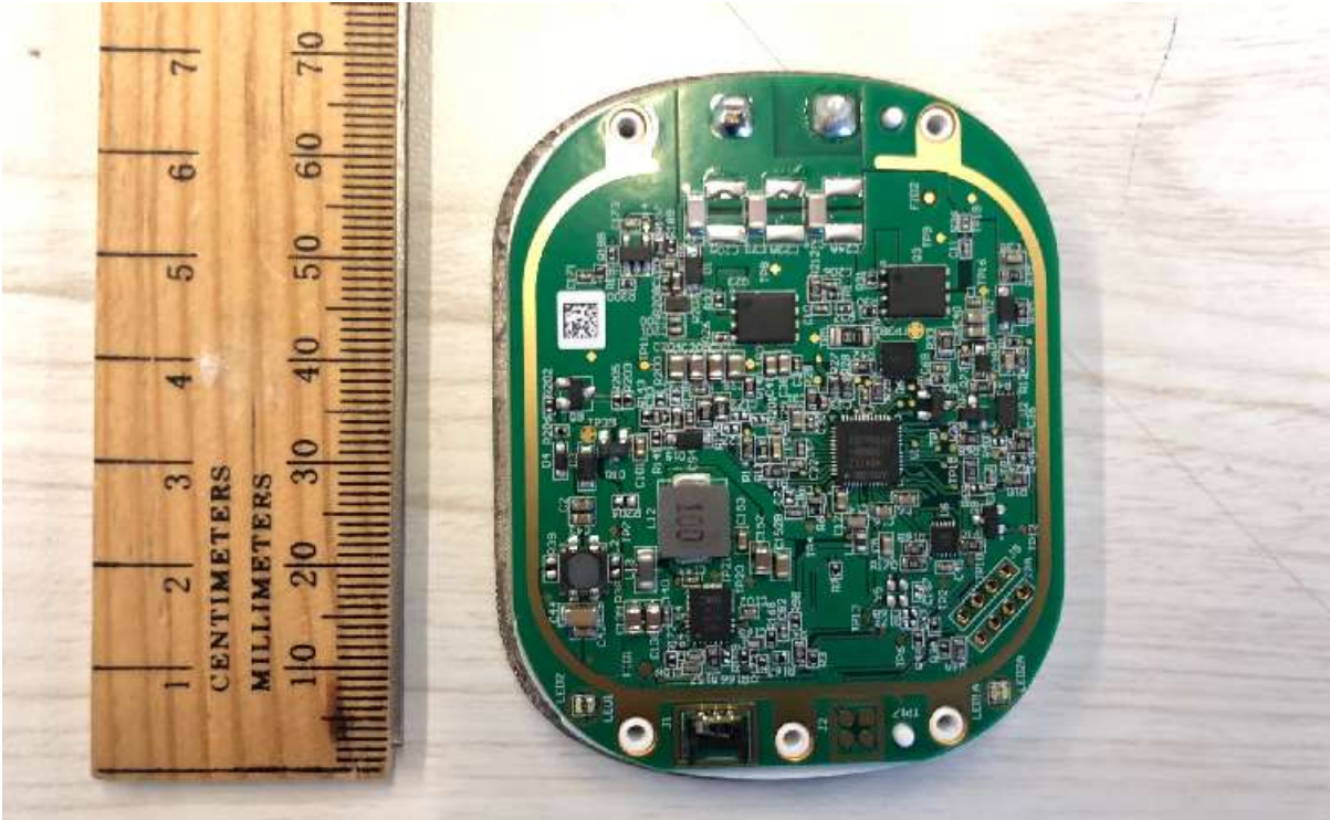
PCB Backside without shield
