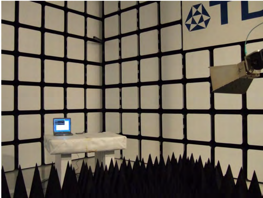
Test Configuration 2: 3 GHz to 5 GHz
