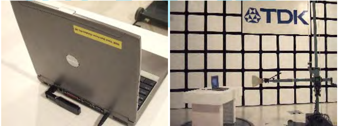
Test Configuration 1. 960 MHz to 40 GHz
