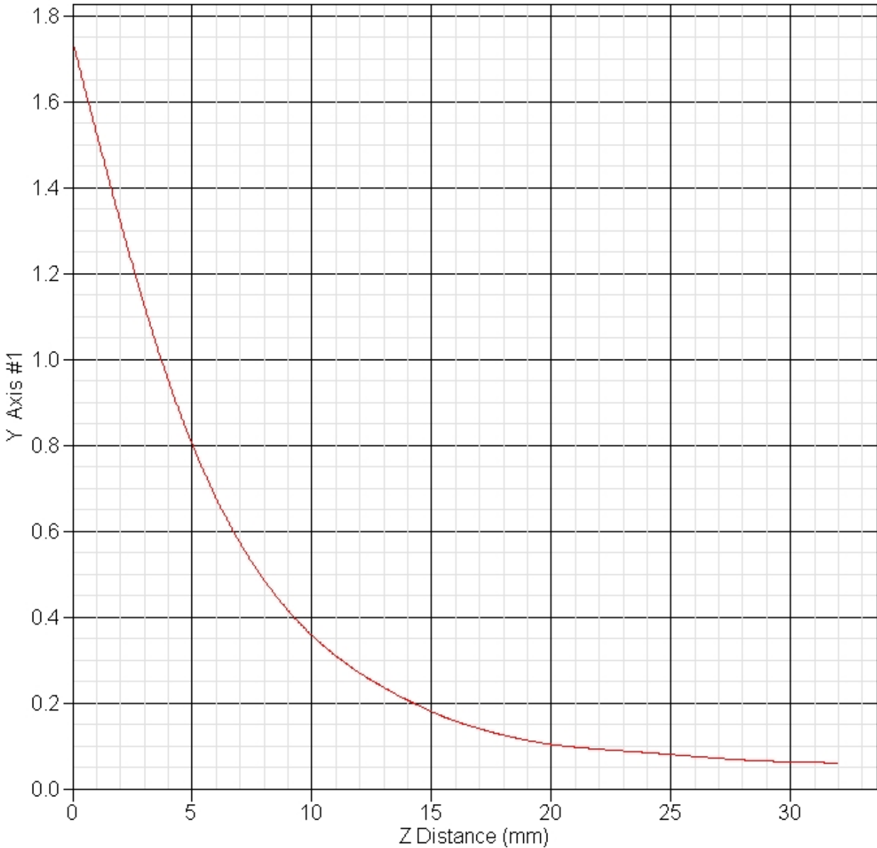
SAR-Z Axis at Hotspot x:-5.80 y:0.00
