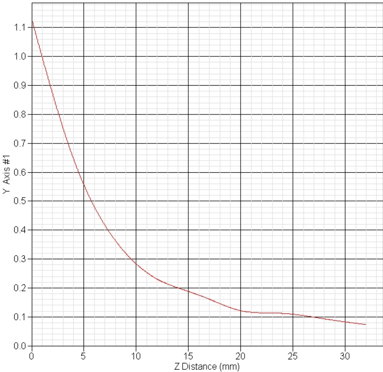
SAR-Z Axis at Hotspot x:0.20 y:5.70
