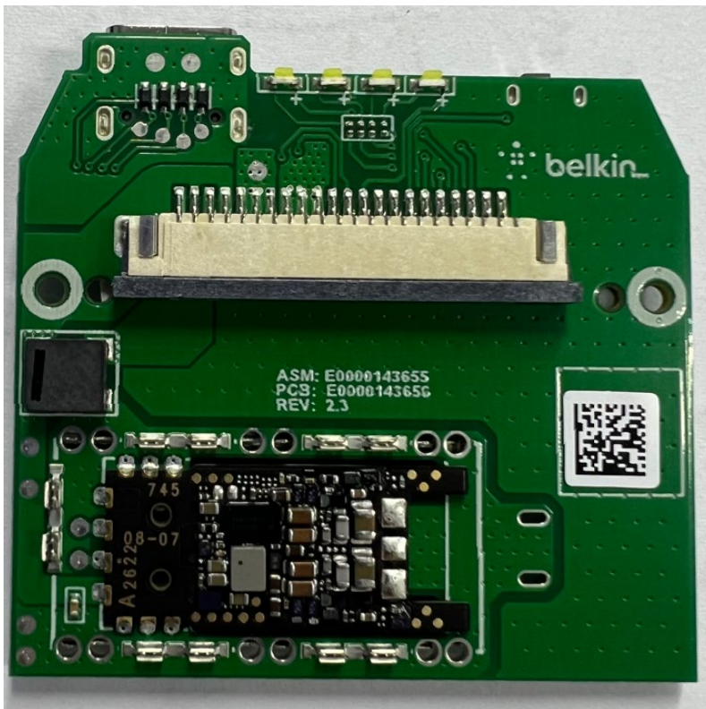
PCBA 2 – Top View (without shielding)
