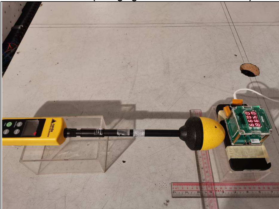
Electric Field (Charging mode with receiver load)
