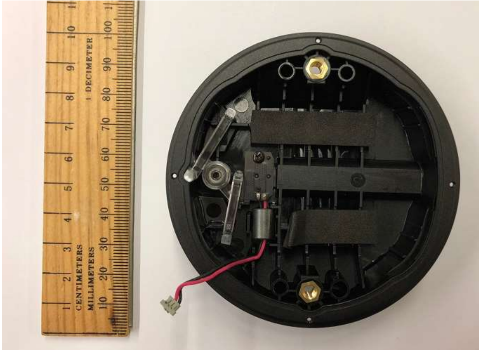
PCB Backside with plastic shield
