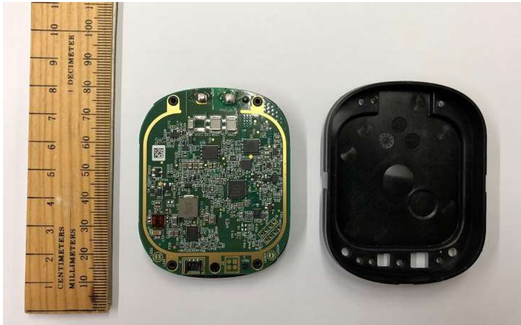
PCB Front side with coil
