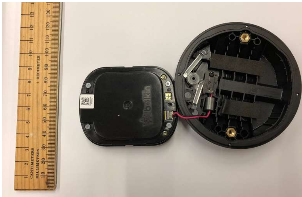
Internal view with coil back and bottom housing
