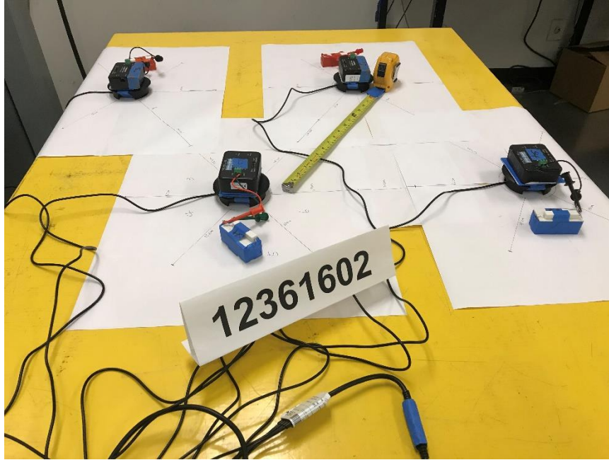
QUAD UNIT WITH FULL CHARGE OF 4X 10W LOADS SETUP PHOTO
