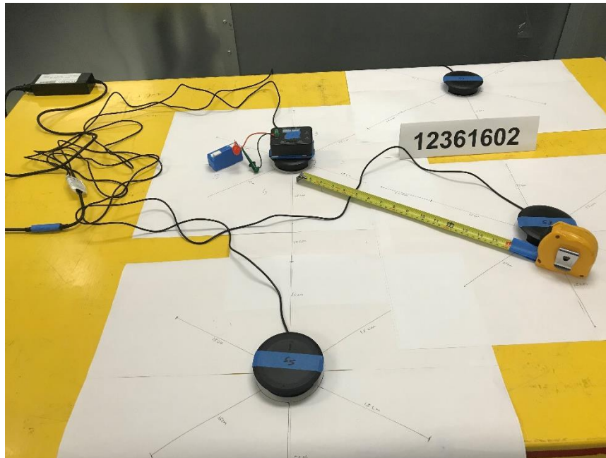
QUAD UNIT WITH SINGLE CHARGE OF 10W LOAD SETUP PHOTO
