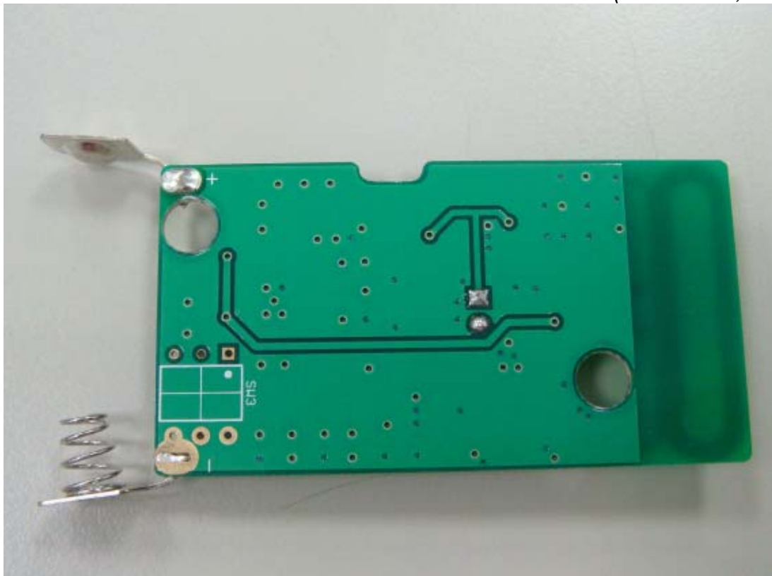
Figure 6 Internal View (Main Board, Back View)
