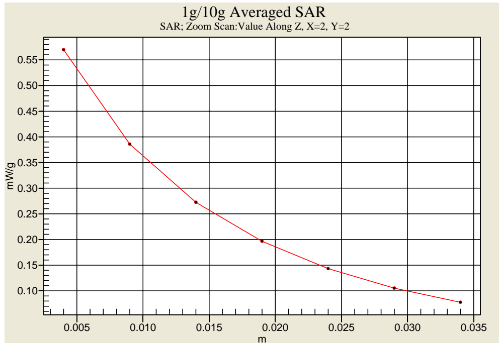
FRS Body SAR with Headset -1.5 cm Spacing _ CH14 _ ALKALINE (2007.08.17)
