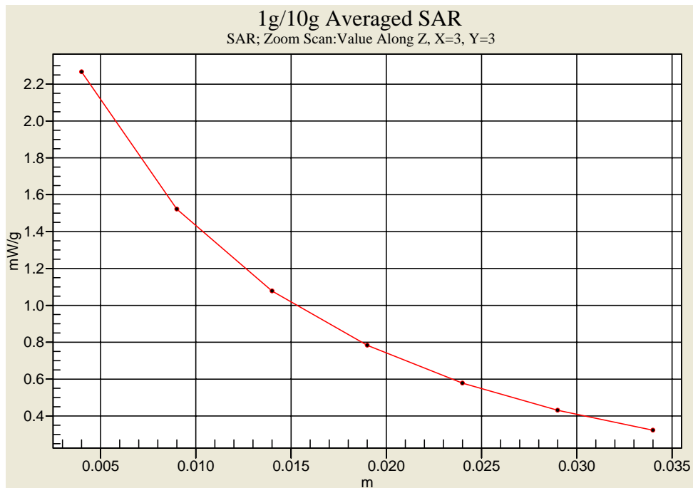
Head-Tissue-Simulating-Liquid 450MHz (2007.09.12)
