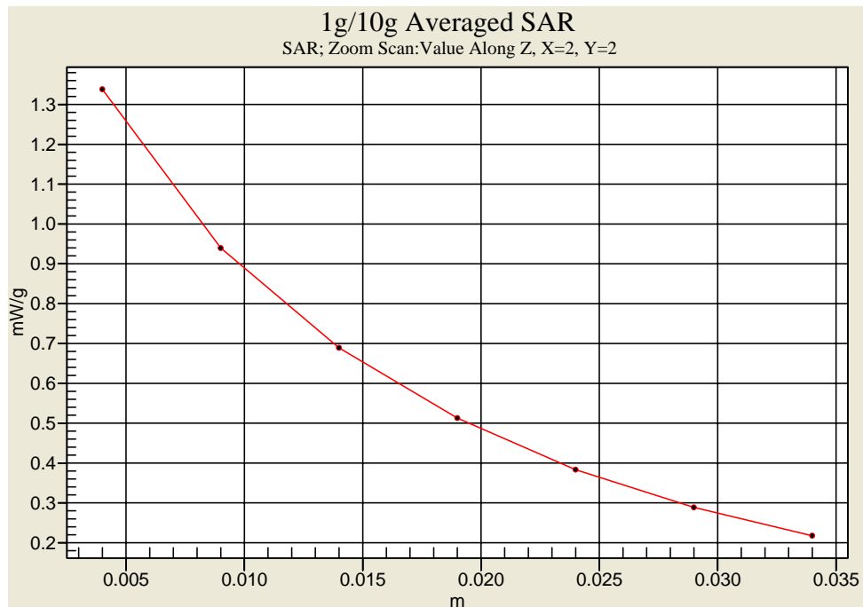
GPRS Body SAR with Headset -1.5 cm Spacing _ CH15 _ ALKALINE ( 2007.08.20 )
