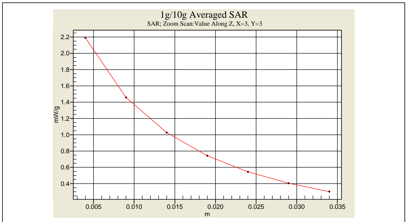
Head -Tissue-Simulating-Liquid 450MHz(2007.08.20)
