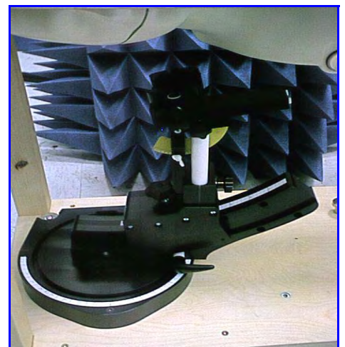
Figure 13. Device Holder
