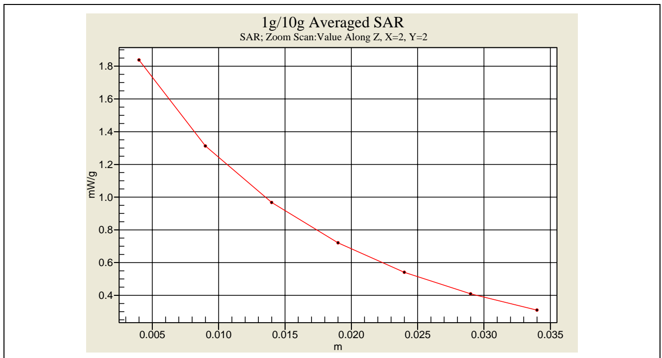
GPRS Head SAR - 1.5 cm Spacing _ CH4 _ ALKALINE ( 2007.08.15 )
