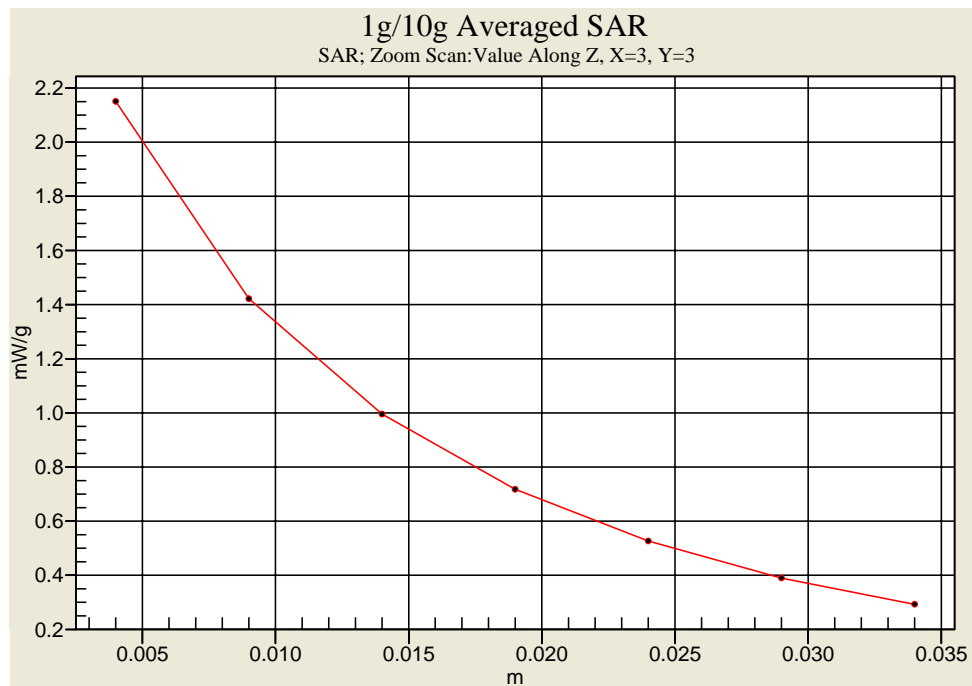
Body-Tissue-Simulating-Liquid 450MHz (2007.08.20)
