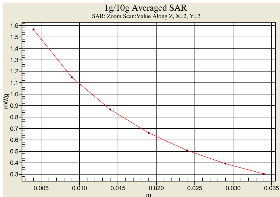
GPRS Head SAR - 1.5 cm Spacing _ CH4 _ ALKALINE ( 2007.09.12 )
