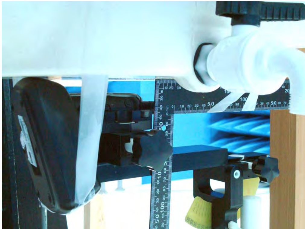
Figure 20. SAR Test Setup Face Position _ with Charger Tray
