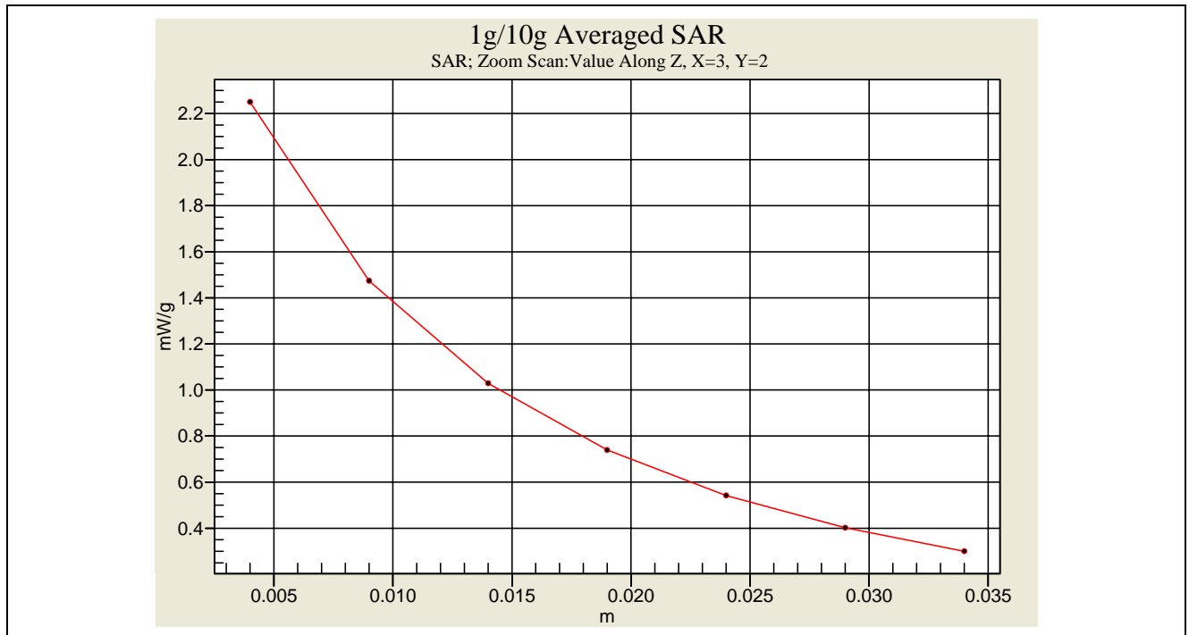
Head-Tissue-Simulating-Liquid 450MHz (2007.08.15)
