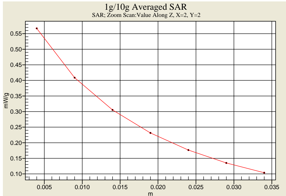
FRS Head SAR -1.5 cm Spacing _ CH11 _ ALKALINE ( 2007.09.12 )
