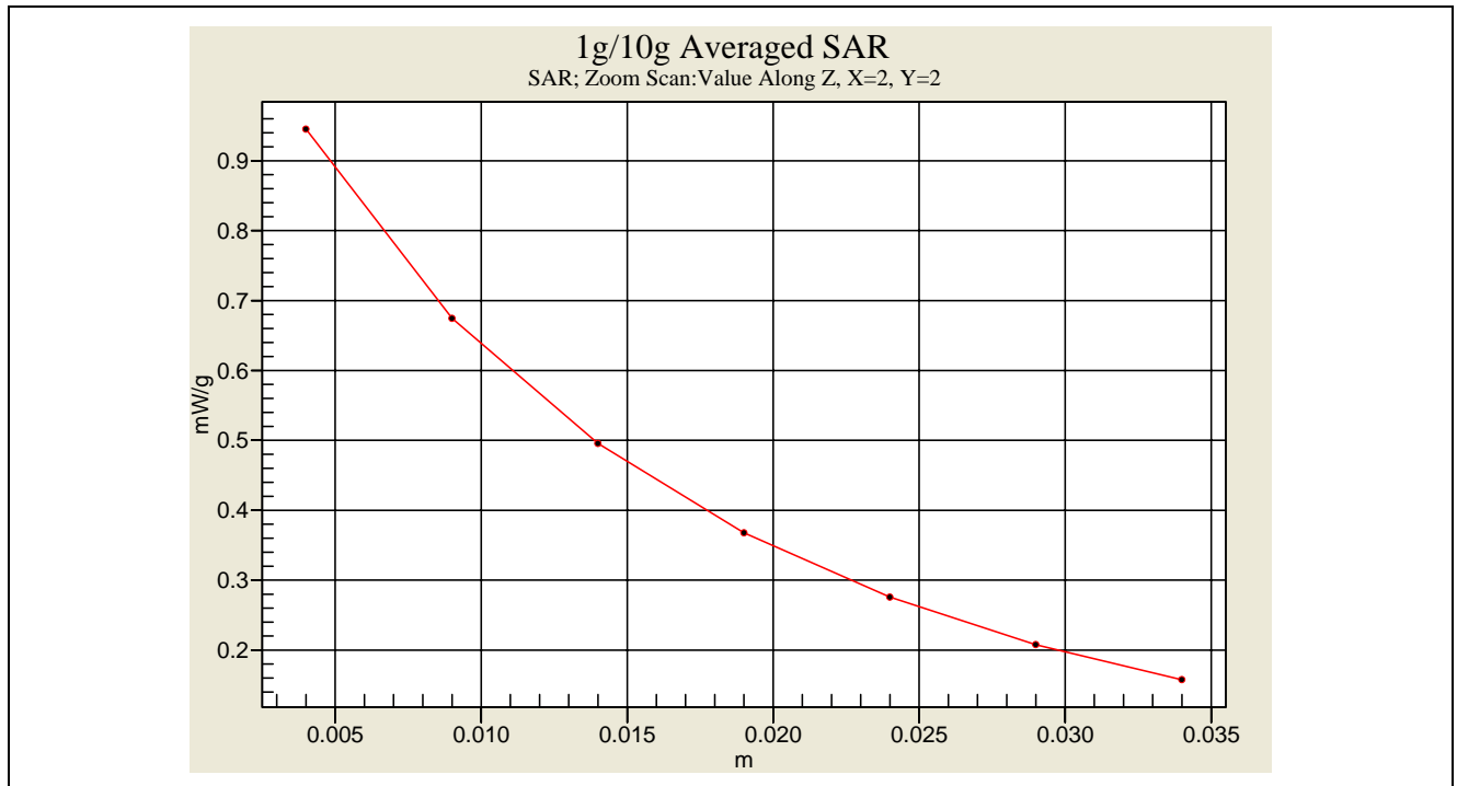
FRS Head SAR -1.5 cm Spacing _ CH11 _ ALKALINE ( 2007.08.15 )
