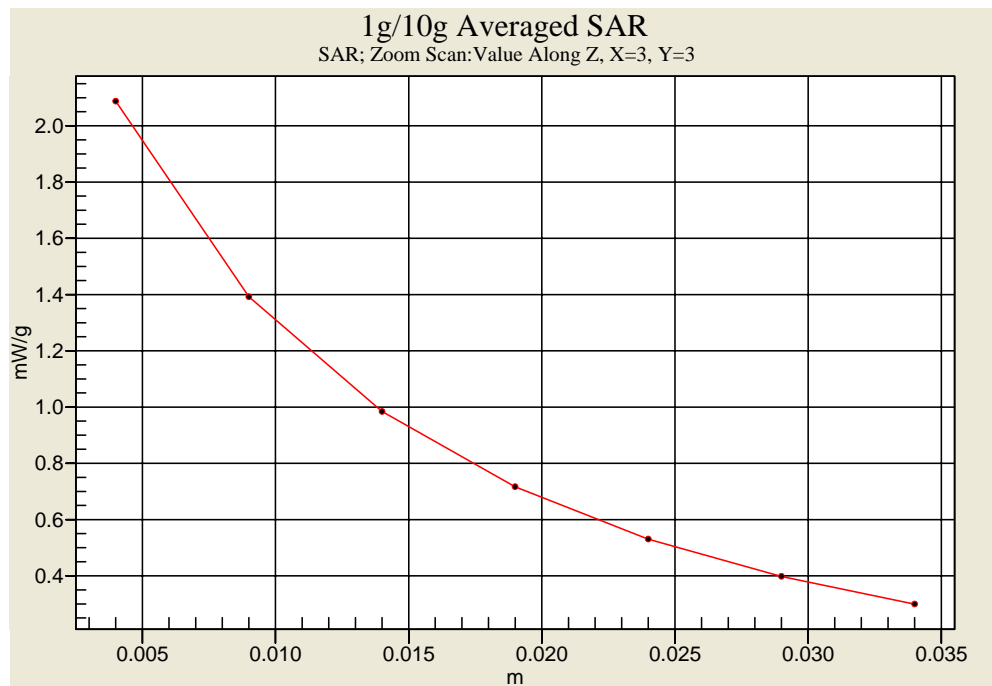
Body-Tissue-Simulating-Liquid 450MHz (2007.08.15)
