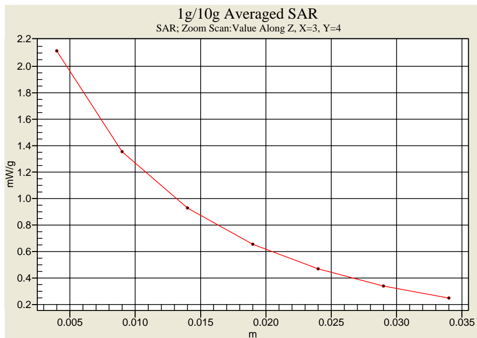
Body-Tissue-Simulating-Liquid 450MHz (2007.08.17)
