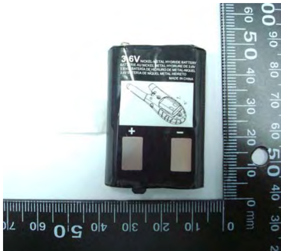
Figure 5. Ni-MH Battery ( 3.6V 700mAh )
