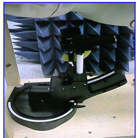
Figure 13. Device Holder
