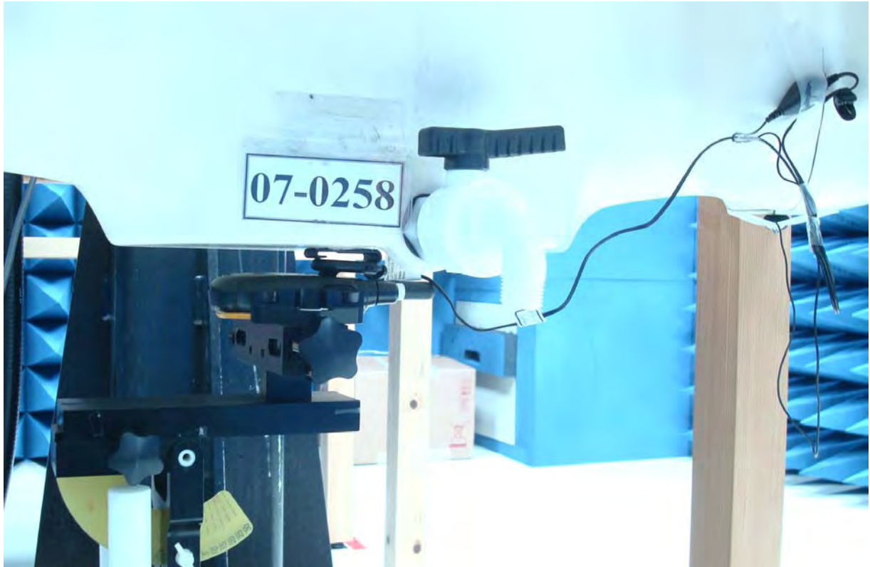
Figure 20. SAR Test Setup with Headset
