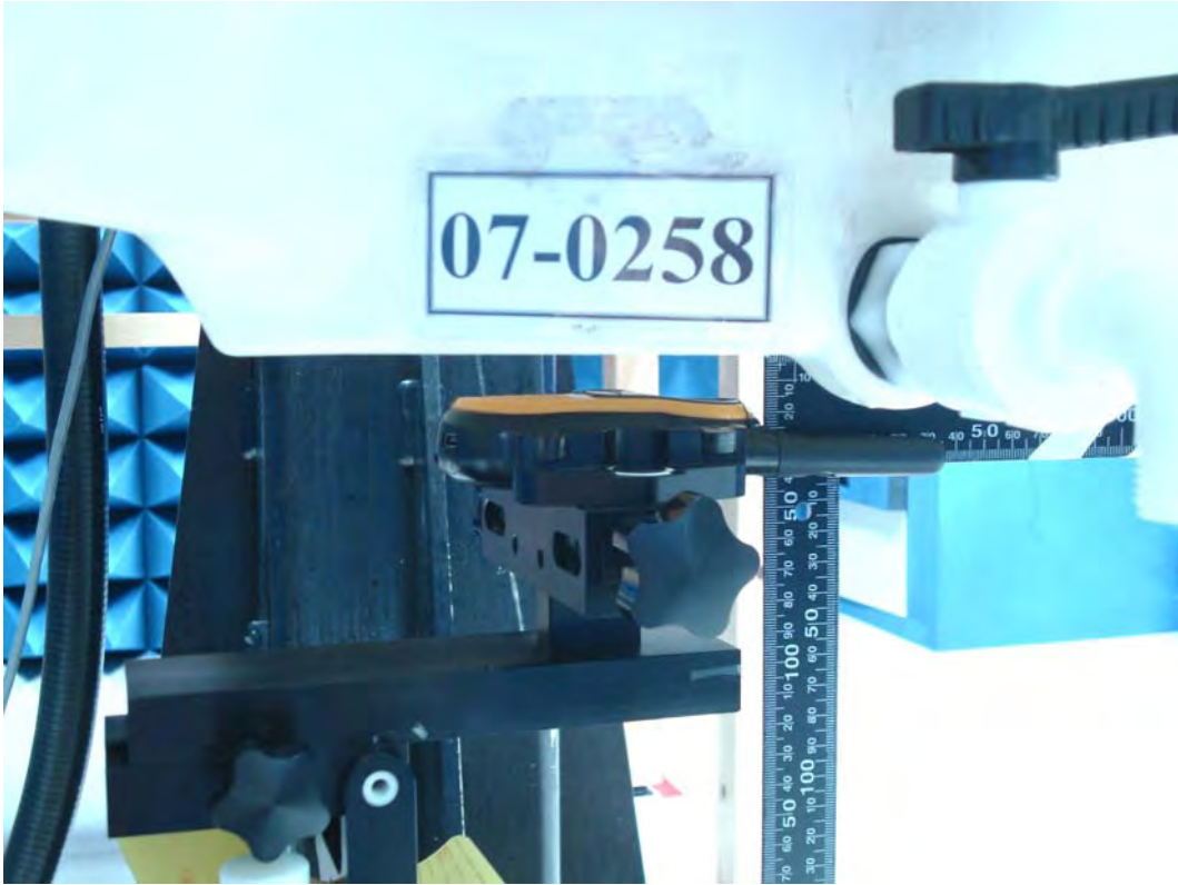
Figure 18. SAR Test Setup Face Position
