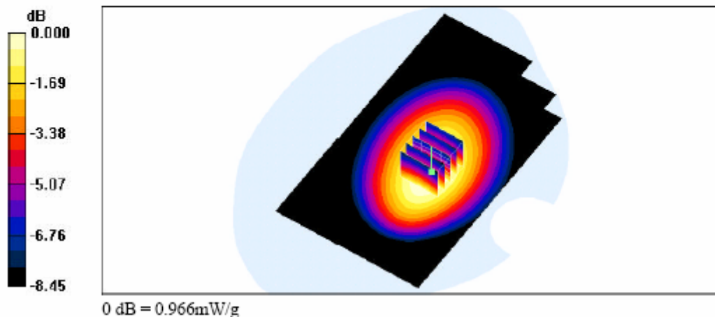
SAR Test Result for GMRS Body SAR w / Belt -clip Channel 22
