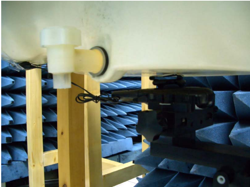
Figure16. SAR Test Setup w/Belt Clip
