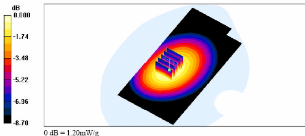
SAR Test Result for GMRS Face SAR -2.5 cm Spacing-Channel 22
