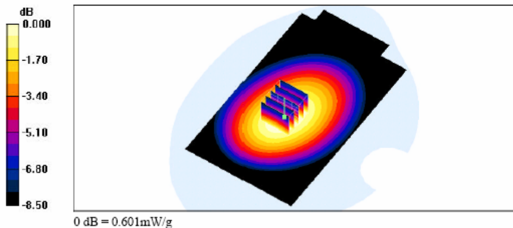
SAR Test Result for FRS Face SAR -2.5 cm Spacing-Channel 11
