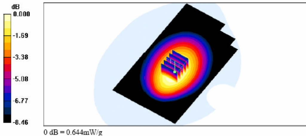
SAR Test Result for FRS Body SAR w / Belt -clip Channel 8
