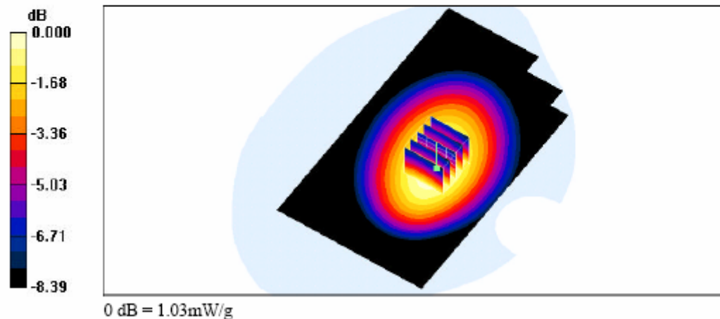
SAR Test Result for GMRS Body SAR w / Belt -clip Channel 4
