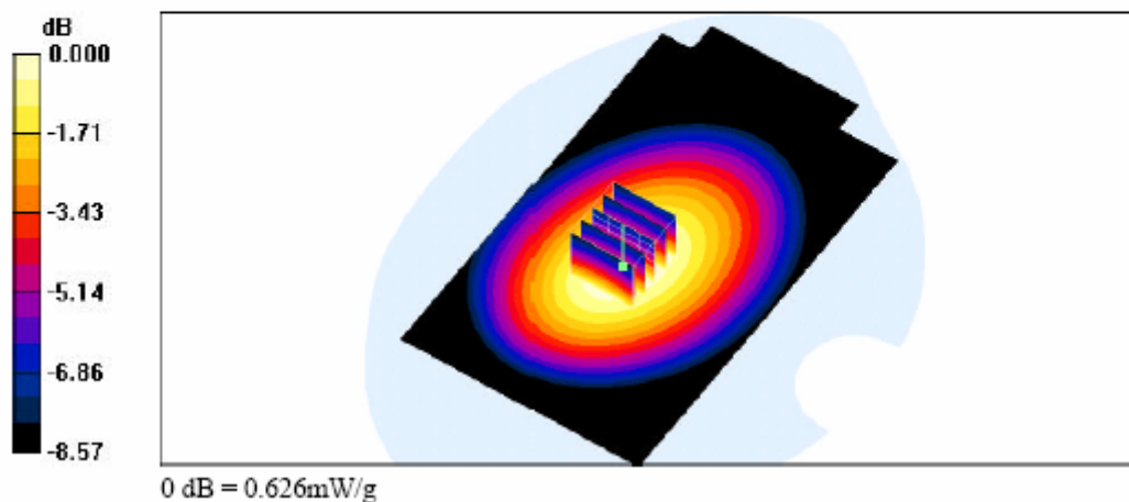
SAR Test Result for FRS Face SAR -2.5 cm Spacing-Channel 8
