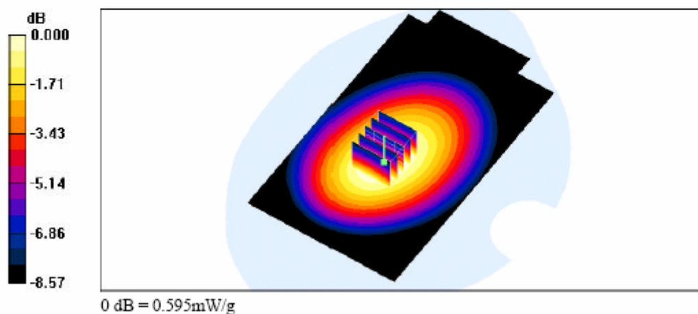
SAR Test Result for FRS Face SAR -2.5 cm Spacing-Channel 14
