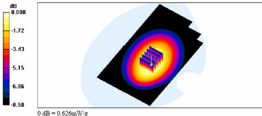
SAR Test Result for FRS Body SAR w / Belt -clip Channel 14
