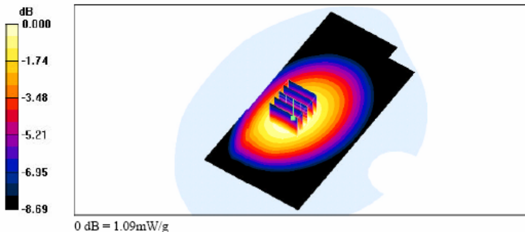
SAR Test Result for GMRS Face SAR -2.5 cm Spacing-Channel 4
