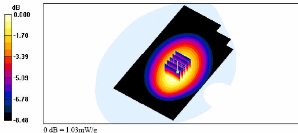
SAR Test Result for GMRS Body SAR w / Belt -clip Channel 15
