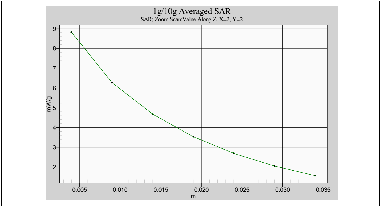
Body SAR with Headset and Belt Clip _ CH16
