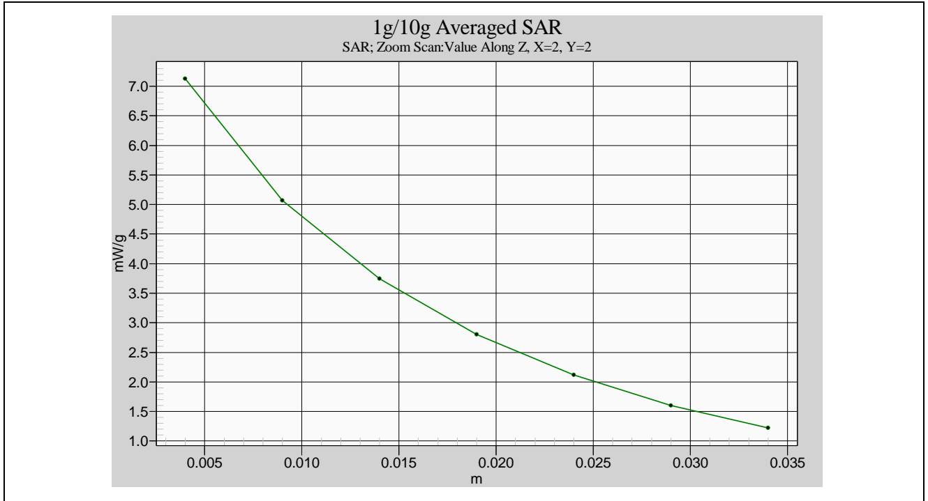
Face SAR -1.5 cm Spacing _ CH16
