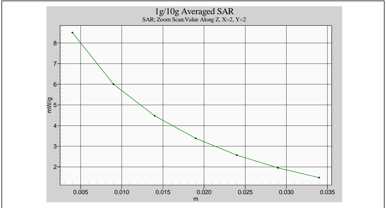
Body SAR with Headset _15 mm Spacing _ CH1
