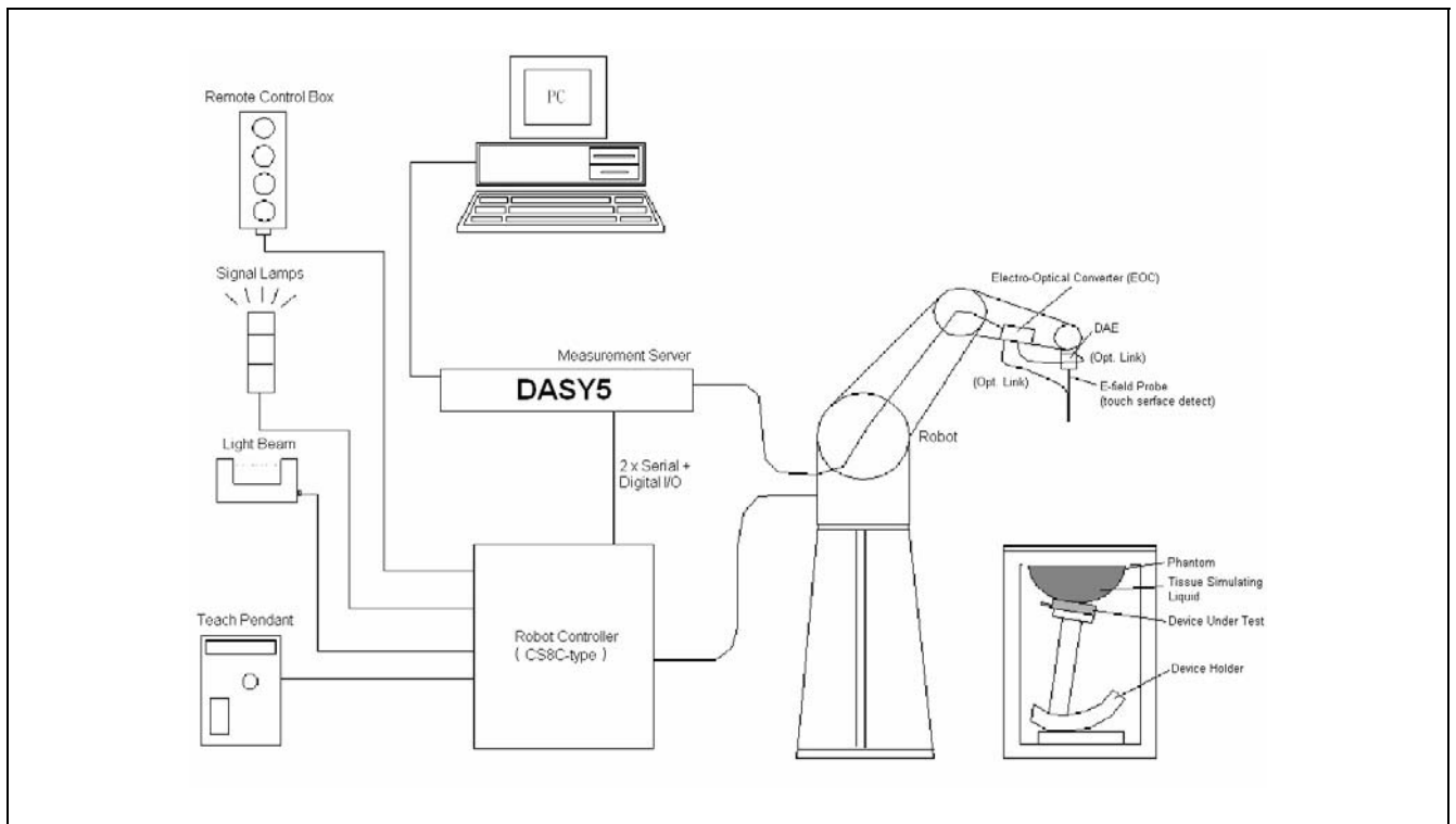
Figure 10. SAR Lab Test Measurement Setup
