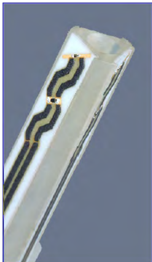
Figure 2. E-field Probe
