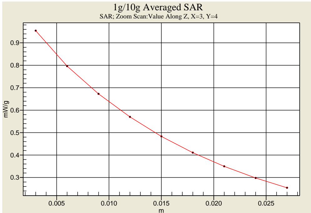
GMRS_CH4 (Ni-MH Battery)
