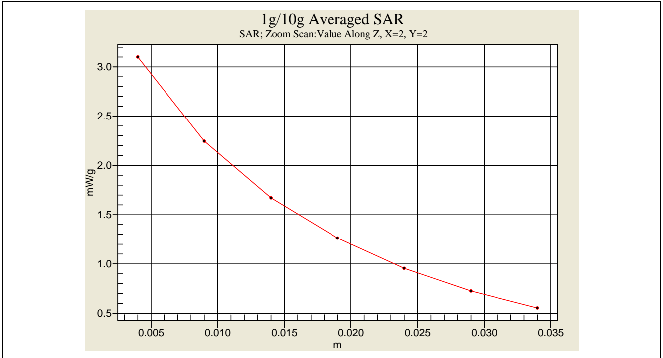
GPRS Head SAR - 1.5 cm Spacing _ CH22_ ALKALINE ( 2007.12.14 )
