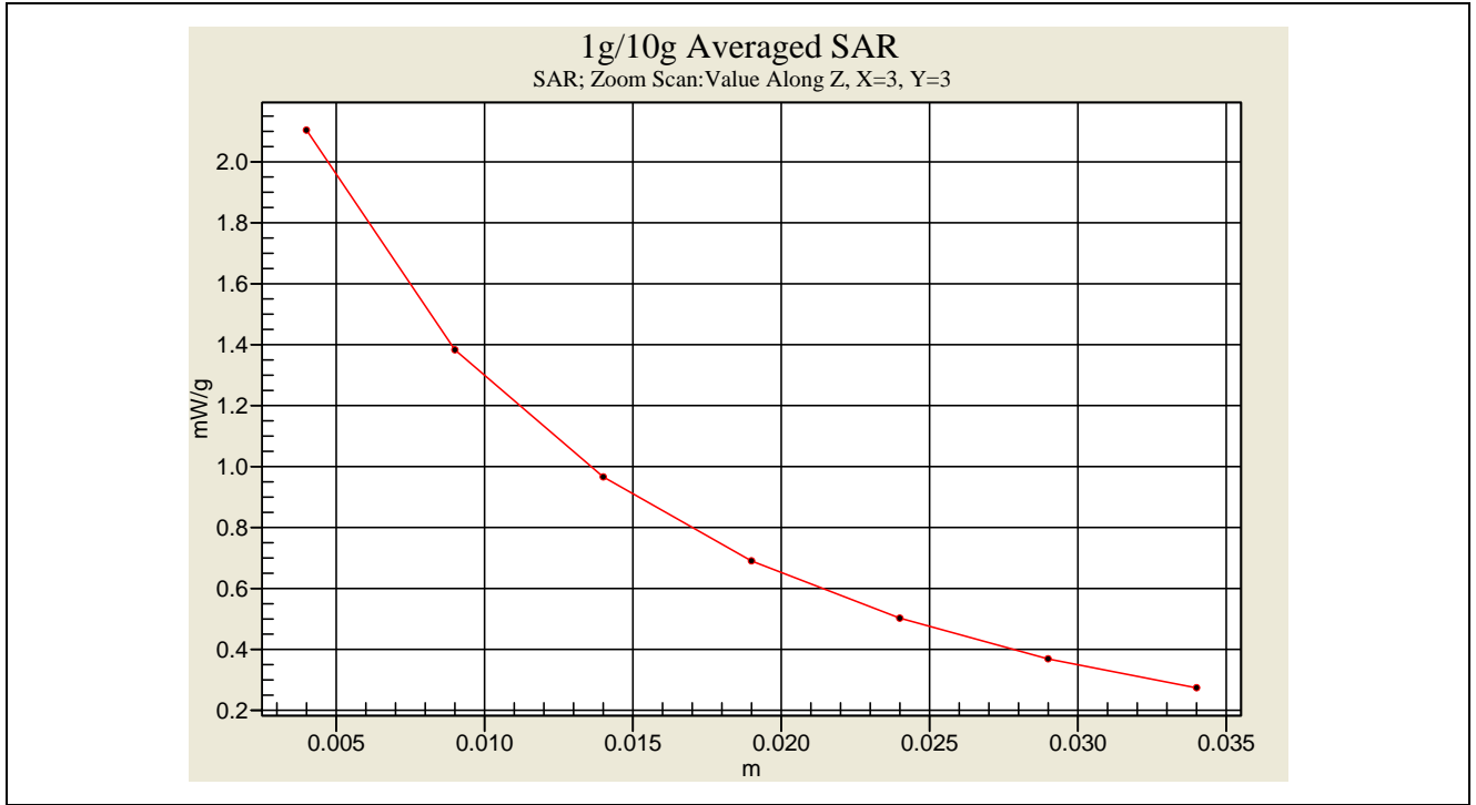
Body-Tissue-Simulating-Liquid 450MHz (2007.12.14)
