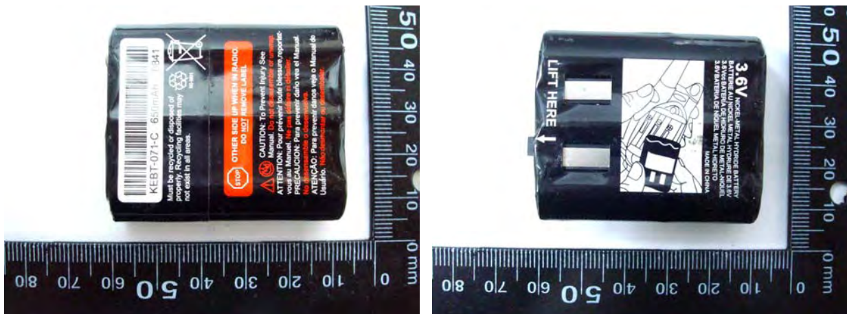
Figure 5. Ni-MH Battery ( 3.6V 650mAh )
