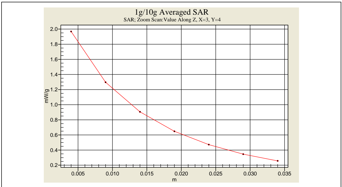
Body-Tissue-Simulating-Liquid 450MHz (2007.12.13)
