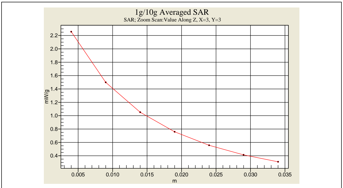
Head -Tissue-Simulating-Liquid 450MHz (2007.12.14)
