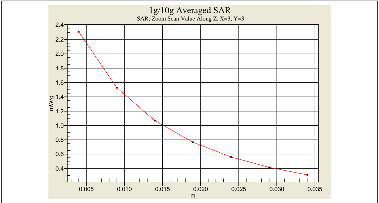
Head-Tissue-Simulating-Liquid 450MHz (2007.12.12)
