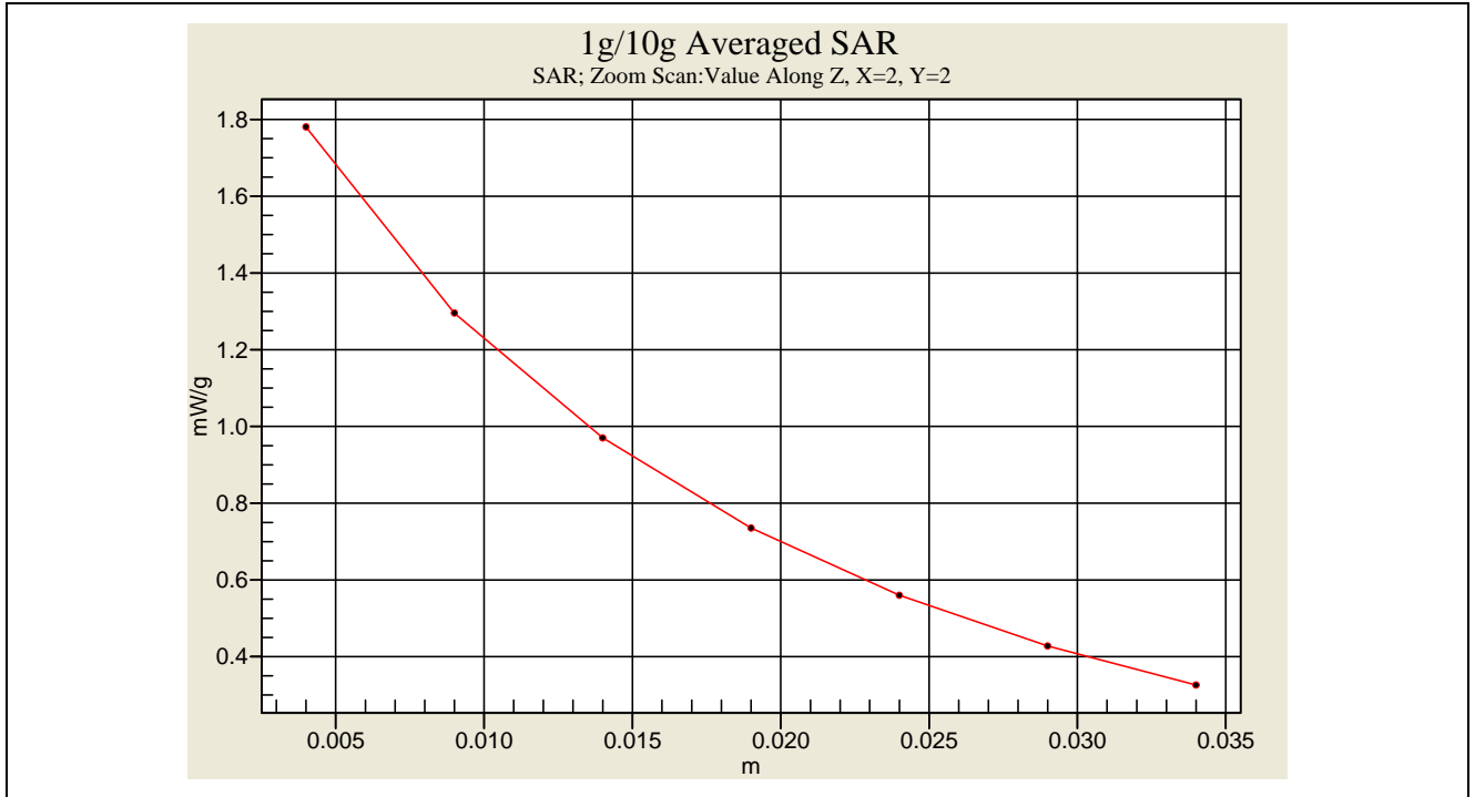
GPRS Body SAR with Headset_Belt Clip -1.5 cm Spacing _ CH22 _ ALKALINE ( 2007.12.14 )
