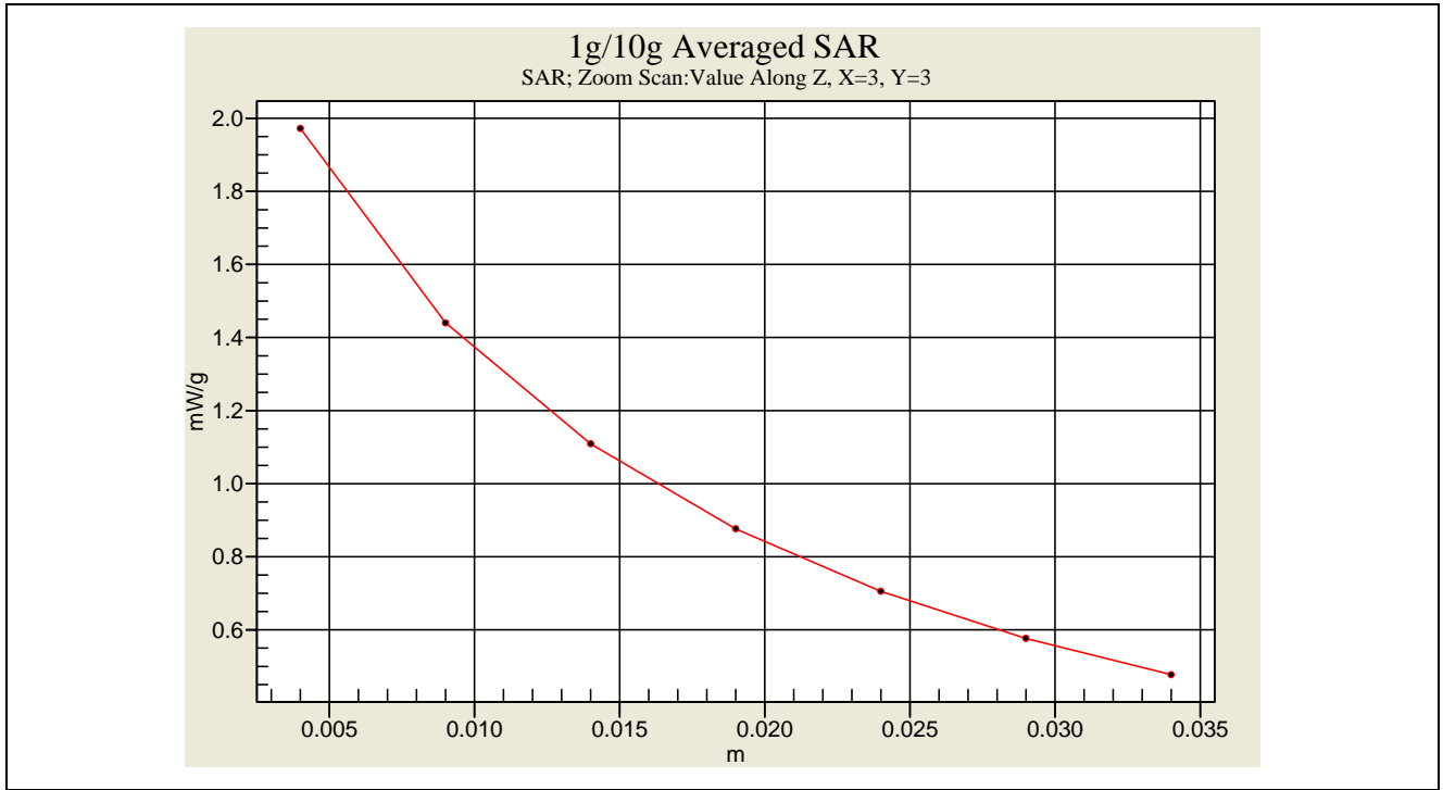
Head -Tissue-Simulating-Liquid 450MHz (2008.12.09)
