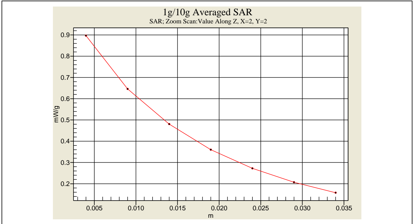
FRS Head SAR -1.5 cm Spacing _ CH8 _ ALKALINE ( 2007.12.12 )
