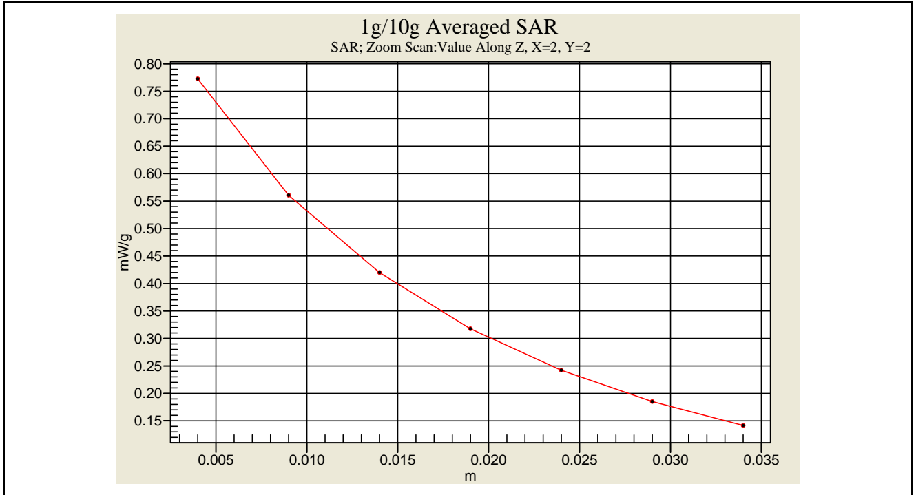
FRS Body SAR with Headset_Belt Clip -1.5 cm Spacing _ CH14 _ ALKALINE (2007.12.14)
