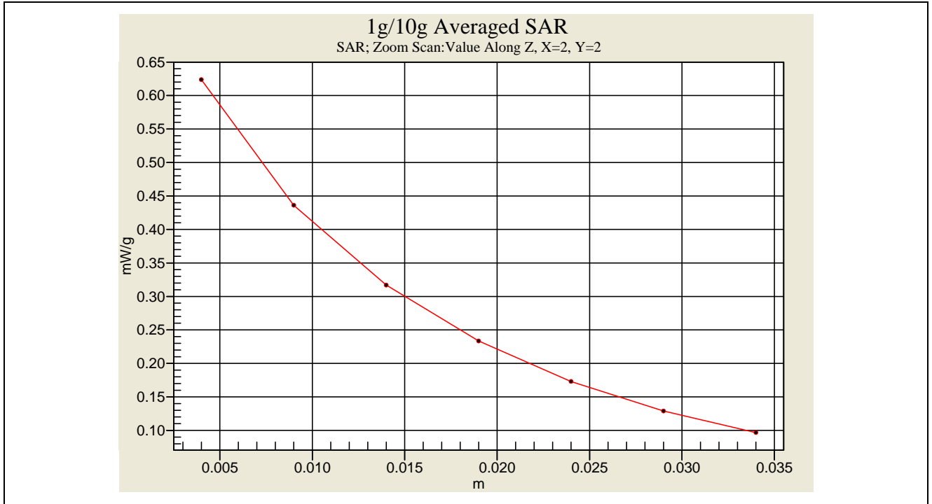
FRS Head SAR -1.5 cm Spacing _ CH14 _ ALKALINE ( 2007.12.13 )
