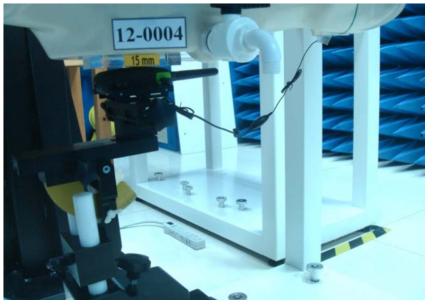
Figure 3. Muscle SAR Test Setup (Flat Section)
