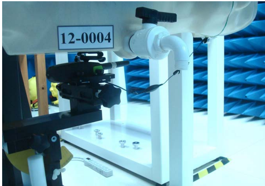
Figure 4. Muscle SAR Test Setup (Flat Section)
