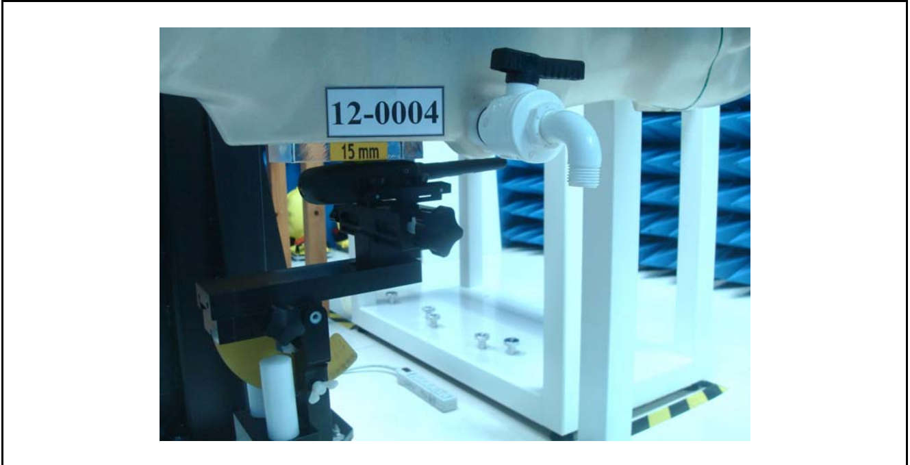
Figure 2. Brain SAR Test Setup (Flat Section)
