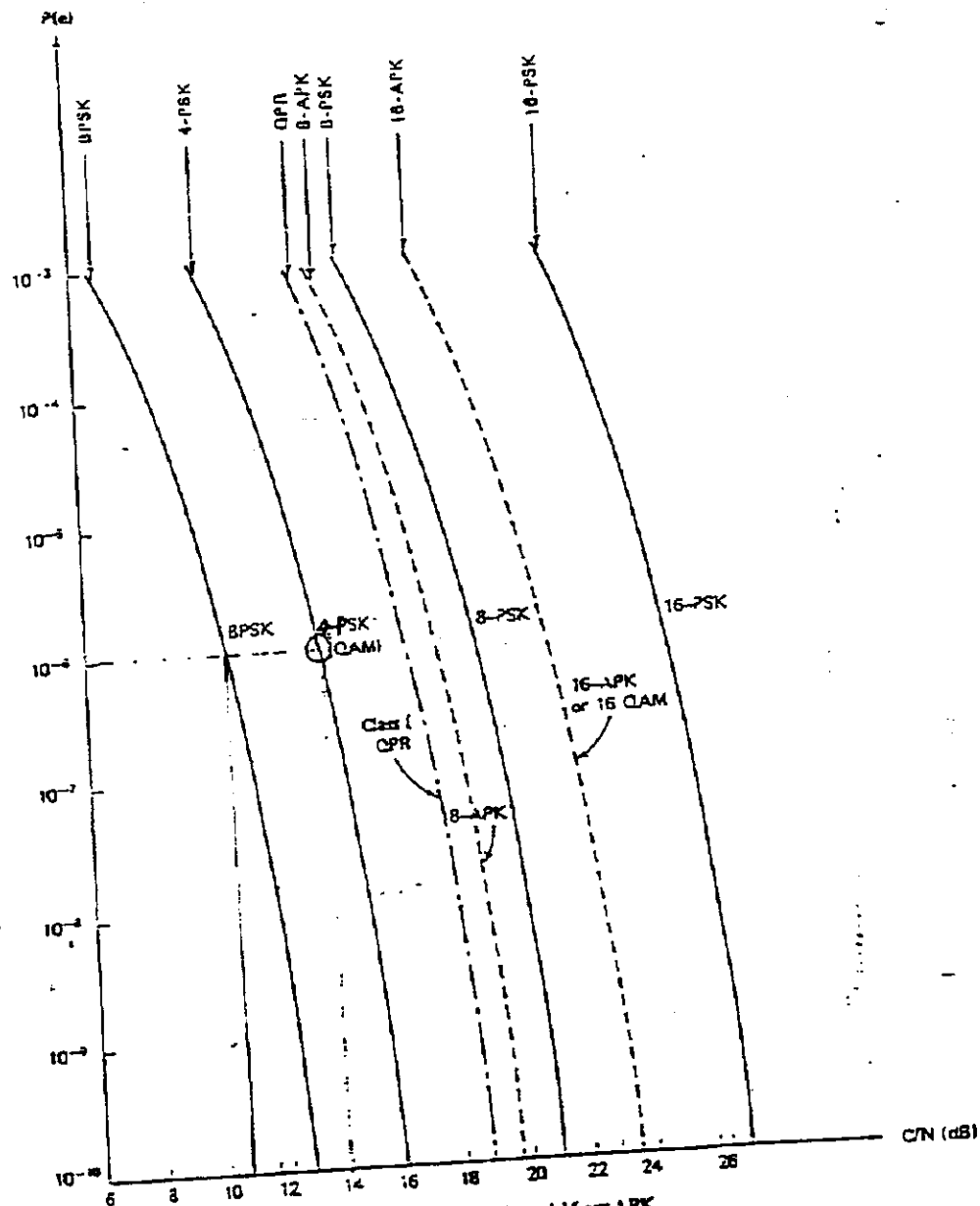
Fig. 3.11. P(e) performance of M -ary PSK, QAM, QPS, and M -ary APK coherent systems. The rms C/N is specified in the double-sided Nyquist bandwidth.
